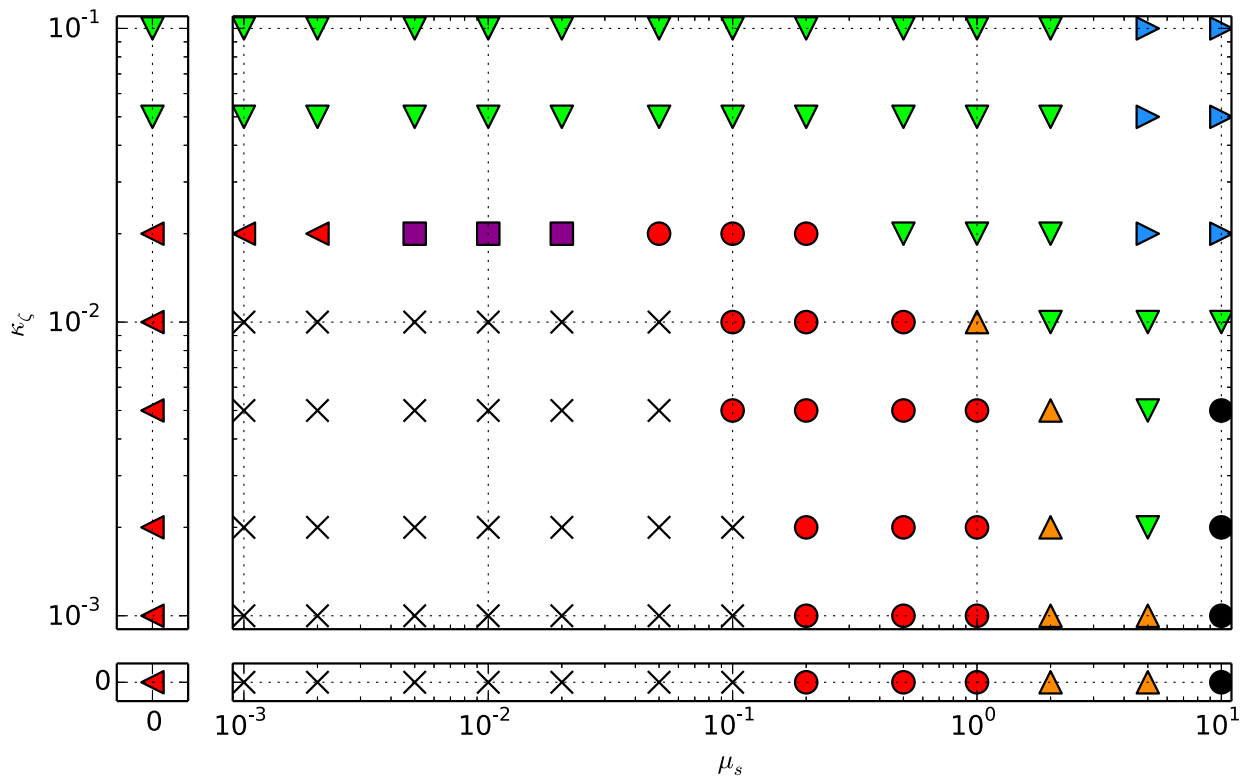
FIGURE 14. Section 5.3.3 Classification of the solution as a function of the (\mu_s, \kappa_\zeta) parameters.
