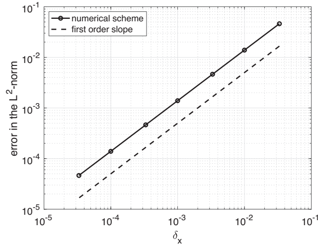
FIGURE 2. Section 4.3.1 Convergence towards an analytical solution.
