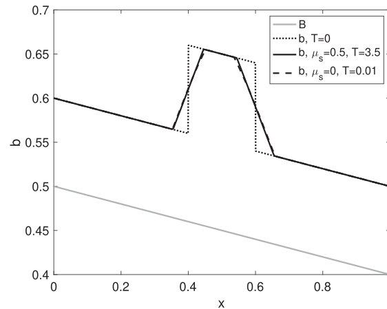
FIGURE 5. Section 4.3.4 Non-flat steady solutions with and without viscosity.
