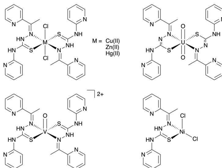
Fig. 69: Heterocyclic TSC ligands complexed with a range of metals and assessed for antifungal properties.
