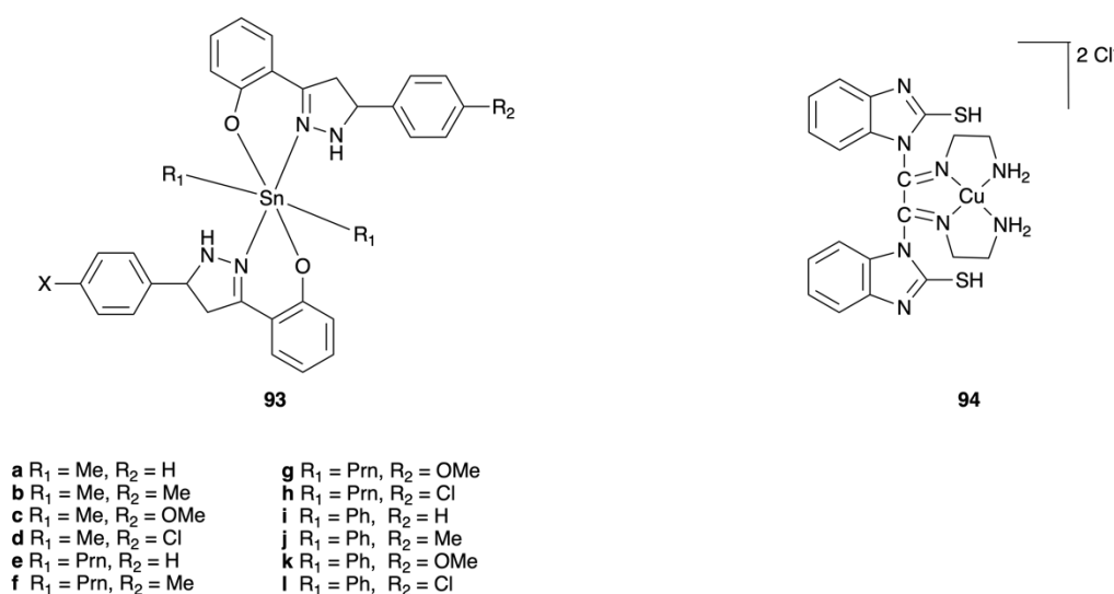
Fig. 29: Metal complexes based on heterocycles assessed for antifungal activity.
