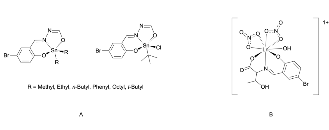
Fig. 55: A Complexes formed between a bromosalicylic hydrazine Schiff base ligand and various organo Sn(IV) sources. B Complex formed between Ln(III) ions and a threonine-bromosalicylic Schiff base ligand; structure not displayed in original article by Logu et al. , but was drawn by the authors of this review from the originally reported spectroscopic data.
