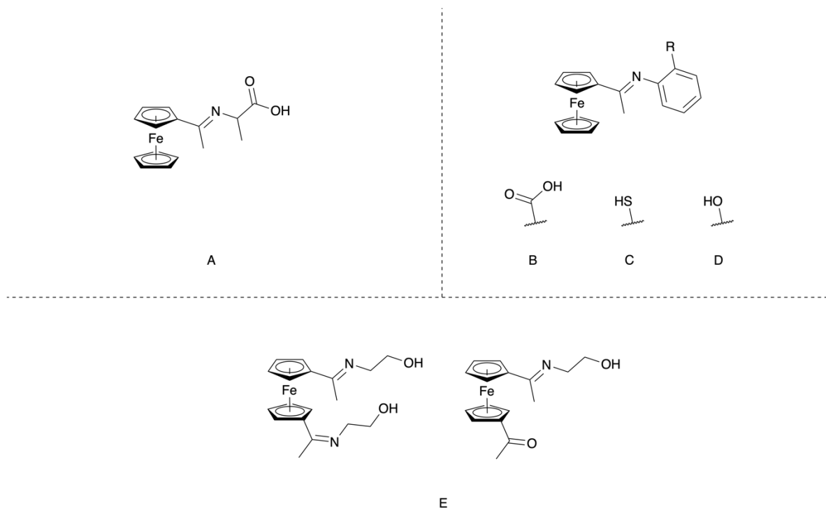
Fig. 58: Ferrocene-containing Schiff base ligands complexed with a range of metals (not shown) and assessed for antifungal properties.
