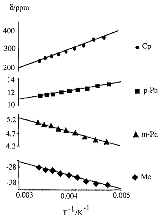
Fig. 1. Chemical shifts for compound 1 as a function of temperature. Solvent = \text{CDCl}_3 .
