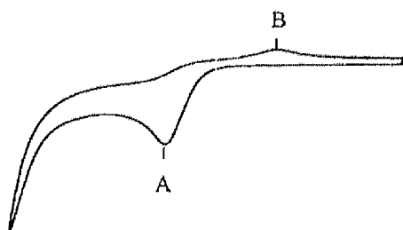
Fig. 2. A typical cyclic voltammogram for compounds \text{CpCrCl}_2\text{L} in \text{CH}_2\text{Cl}_2 (see Table 1 for the list of L ligands and potentials for waves A and B).
