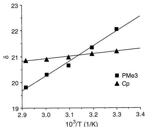
Fig. 1 Temperature dependence of the contact-shifted resonances for compound 1 . Solvent = C_6D_6
