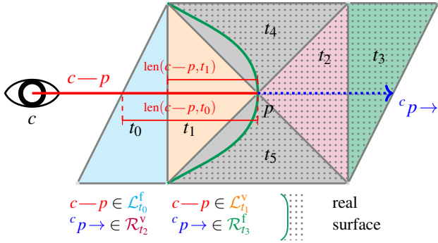
Figure 3: Visibility Model. 2D representation of our visibility features. A line-of-sight c-p between a camera c and a visible 3D point p also defines a ray {}^c p \rightarrow . The line-of-sight c-p traverses the two outside tetrahedra t_0 and t_1 , while the ray {}^c p \rightarrow traverses the two inside tetrahedra t_2 and t_3 . Neither c-p , nor {}^c p \rightarrow traverse t_4 or t_5 ; they thus do not contribute to their visibility information.
