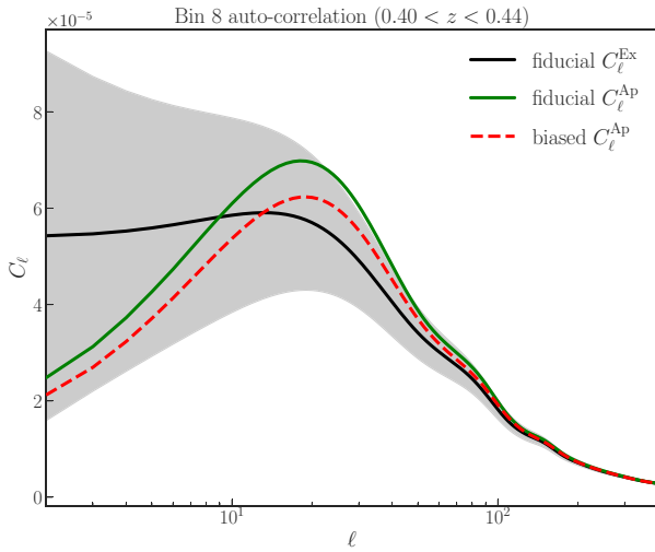
Figure 6. Angular power spectra for the eighth redshift bin autocorrelation in a \Lambda\text{CDM} cosmology using the exact C_\ell^{\text{Ex}} (black solid curve) and the approximated C_\ell^{\text{Ap}} (green solid curve) obtained assuming the fiducial values for the cosmological parameters. The red dashed curve shows the C_\ell^{\text{Ap}} obtained for the biased parameter estimation of Table 3. The grey area shows the errors corresponding to the experimental setup used throughout the paper.
