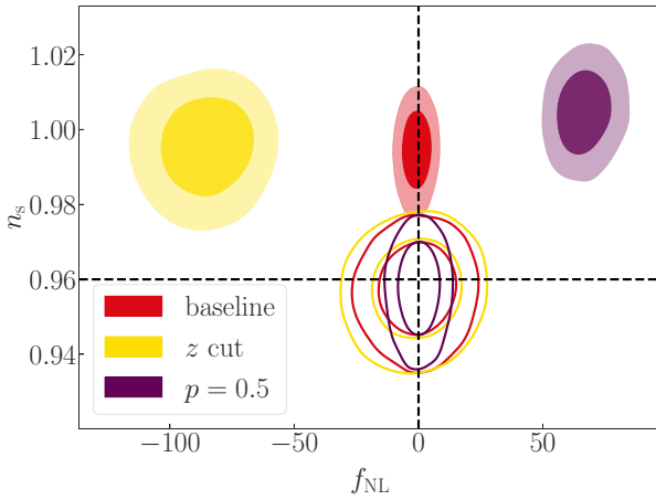
Figure 8. 68 per cent and 95 per cent confidence level contours obtained by fitting the approximated C_\ell^{\text{Ap}} spectra, with a free f_{\text{NL}} parameter, to the data set built using the exact C_\ell^{\text{Ex}} spectra (colour-filled contours). The red and yellow contours show the results obtained with the scale-dependent bias of equation (22), with our baseline settings and with removing the last two redshift bins, respectively. The violet contour shows instead the case where the scale-dependent bias is computed following equation (23) with p = 0.5 . The empty contours show the results of the analysis when the debiasing term described in Section 5.1 is included. The black dashed lines show the values of the fiducial cosmological parameters.
