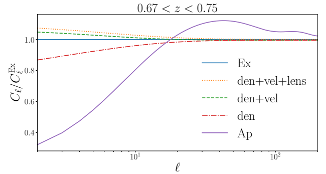
Figure 1. Ratio of the approximated C_\ell to the exact C_\ell^{Ex} of equation (16). The labels of the different curves correspond to the contributions that enter the window function in equation (10). None of the spectra considered here use the Limber approximation, except the ‘Ap’ spectrum, which corresponds to the fully approximated C_\ell^{Ap} of equation (19). The spectra shown here refer to the autocorrelation in a redshift bin with 0.67 < z < 0.75 , using the survey specifications discussed in Section 3.
