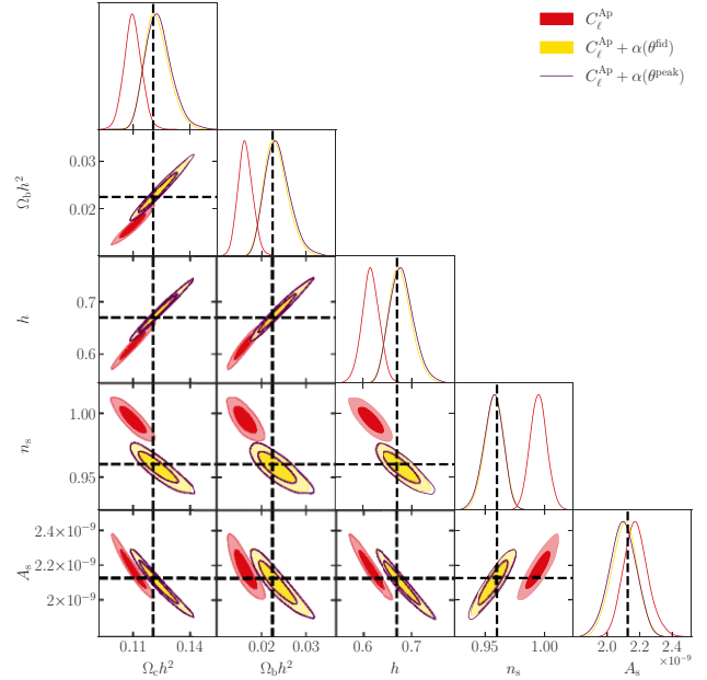
Figure 7. 68 per cent and 95 per cent confidence level contours, as well as one-dimensional marginalized posterior probability distribution functions, obtained by fitting the \Lambda\text{CDM} model to the mock data set. The red, filled contours correspond to the analysis where the theoretically predicted approximated spectra C_\ell^{\text{AP}} are used to fit the model to the mock data set. The yellow, filled contours show the results obtained when the debiasing term \alpha(\Theta^{\text{fid}}) is included, and the purple, empty contours correspond to the debiasing term \alpha(\Theta^{\text{peak}}) computed at the estimated maximum likelihood point \Theta^{\text{peak}} .
