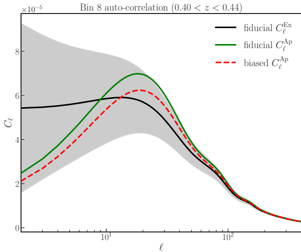
Figure 6. Angular power spectra for the eighth redshift bin autocorrelation in a \Lambda\text{CDM} cosmology using the exact C_\ell^{\text{Ex}} (black solid curve) and the approximated C_\ell^{\text{AP}} (green solid curve) obtained assuming the fiducial values for the cosmological parameters. The red dashed curve shows the C_\ell^{\text{AP}} obtained for the biased parameter estimation of Table 3. The grey area shows the errors corresponding to the experimental setup used throughout the paper.
