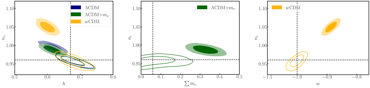
Figure 5. 68 per cent and 95 per cent confidence level contours obtained by fitting the approximated C_\ell^{\text{AP}} spectra to the data set built using the exact C_\ell^{\text{Ex}} spectra (colour-filled contours). The violet contours show the result when a \Lambda\text{CDM} model is assumed, while the green and orange contours correspond instead to \Lambda\text{CDM}+m_\nu and w\text{CDM} cosmologies, respectively. The empty contours show the results of the analysis when the debiasing term described in Section 5.1 is included. The black dashed lines show the fiducial values of the cosmological parameters.
