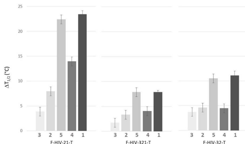
Fig. 3. Thermal stabilization of G4 structures by porphyrins 1 to 5 . Thermal stabilization of the F-HIV-21-T (parallel, left), F-HIV-321-T (anti-parallel, middle) and F-HIV-32-T (hybrid, right) oligonucleotides measured by FRET melting assays. Porphyrin derivatives were added at 2 mol. equivalents (0.4 \mu M) with respect to oligonucleotide (0.2 \mu M) in 10 mM lithium cacodylate buffer pH 7.2, 100 mM KCl. The \Delta T_{1/2} value indicates the difference of melting temperature induced by the ligand.
