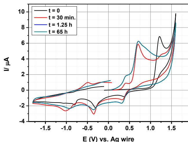
Figure 8. Cyclic voltammograms of A-D-A0 over time in DMSO solutions at room temperature.
