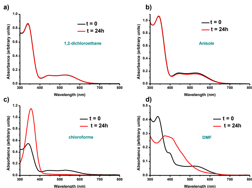
Figure 6. Evolution of the UV-visible spectra of A-D-A0 in different solvent over time.
