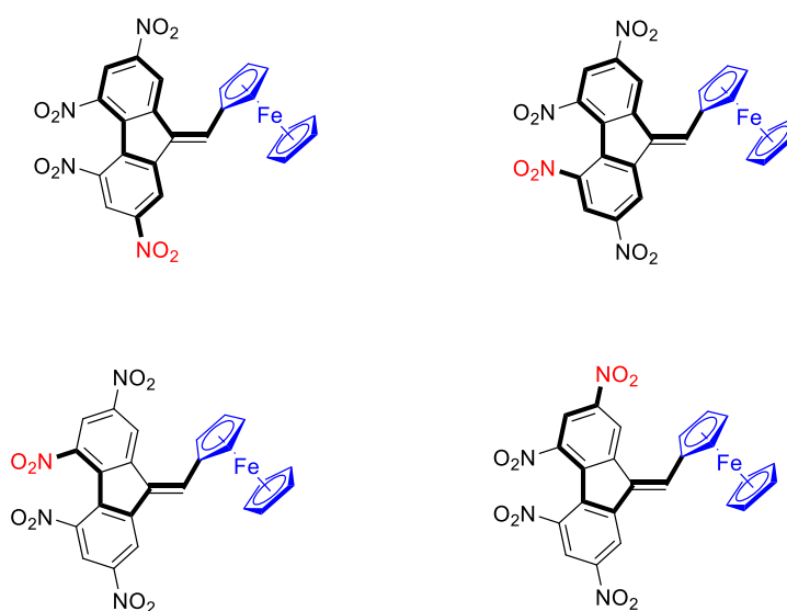
Figure 13. The different mesomeric forms supporting the presence of two ICT bands for the TNF-based dye D-A9 .
