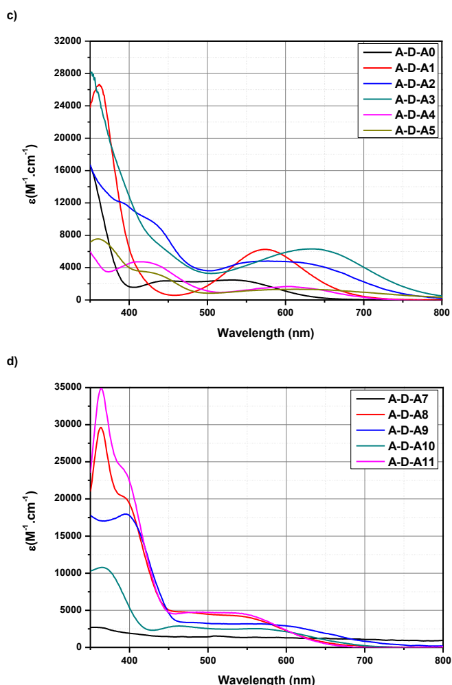
Figure 3. UV-visible absorption spectra of D-A dyads D-Ax , x = 0-11 (a and b) and A-D-A triads A-D-Ax , x = 0-11 (c and d) in chloroform.
