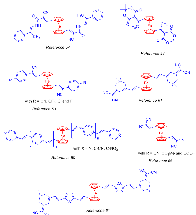
Figure 1. Chemical structures of A-D-A ferrocene triads reported in the literature.
