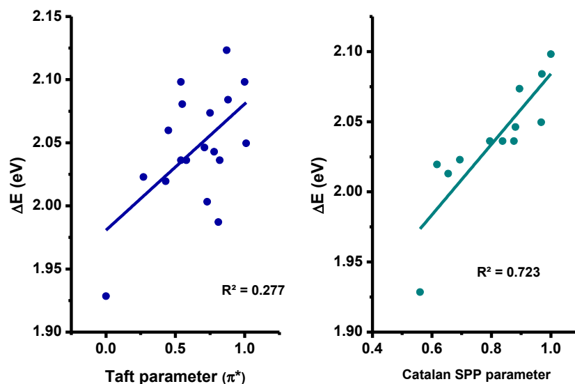
Figure 12. Linear correlations obtained for D-A5 using the Kamlet-Taft and the Catalan empirical scales.
