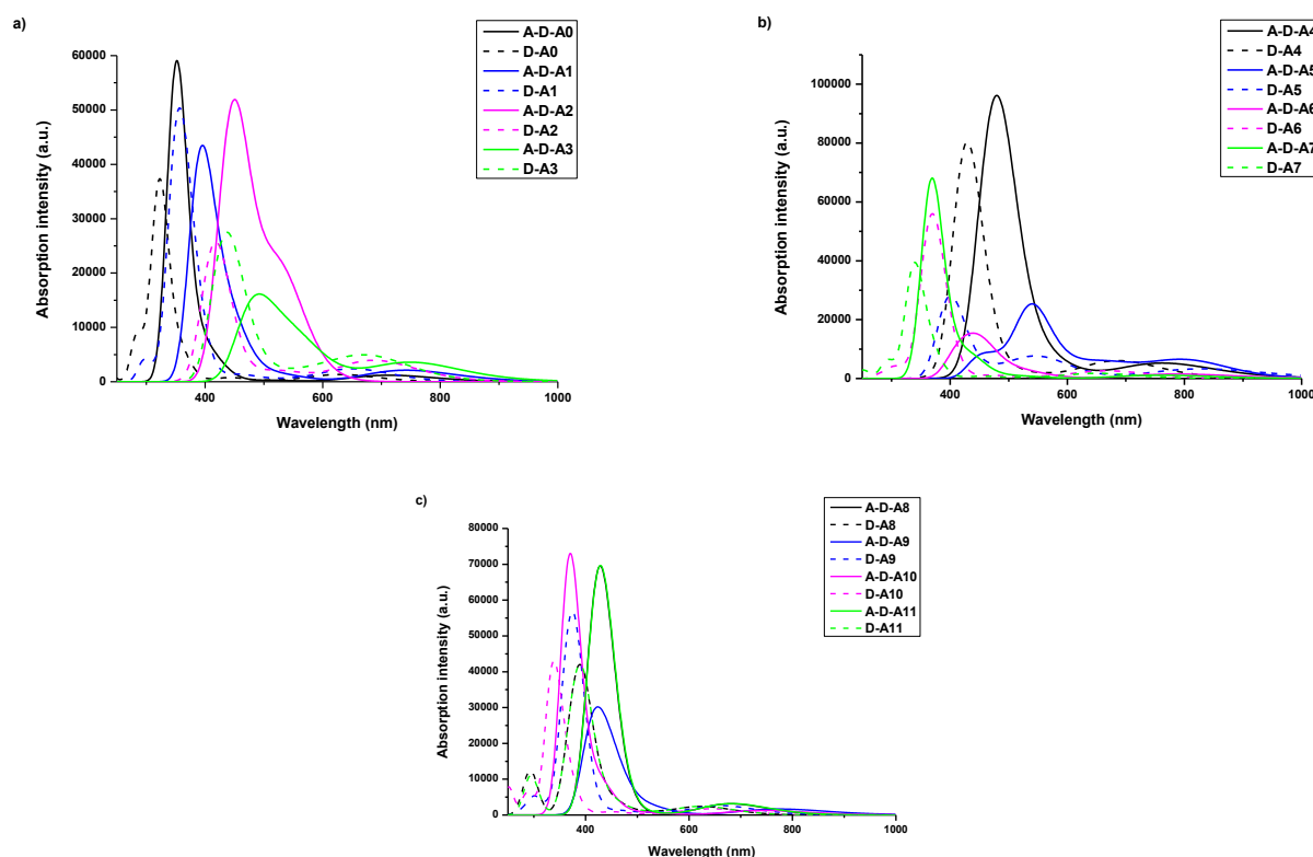
Figure 5. Simulated absorption spectra of D-A dyads D-Ax , x = 0–11 and A-D-A triads A-D-Ax , x = 0–11 in dichloromethane.
