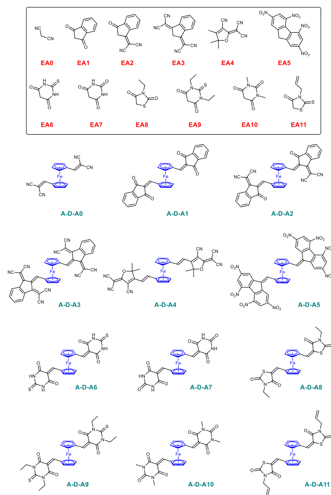
Figure 2. Chemical structures of electron acceptors EAx , x = 0-11 and A-D-A triads A-D-Ax , x = 0-11 .
