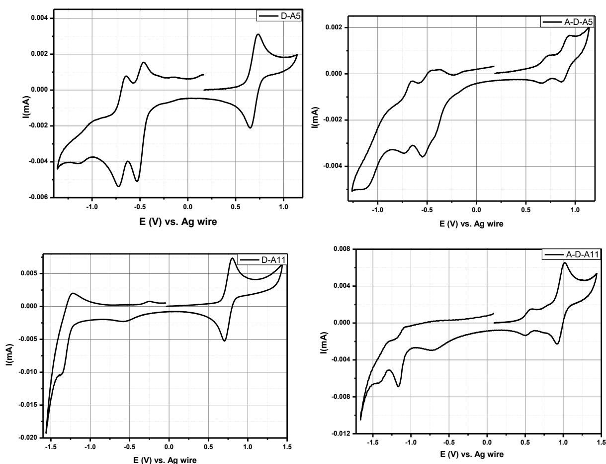
Figure 15. Comparisons between the cyclic voltammograms of D-A5/A-D-A5 (up) and D-A11/A-D-A11 (down) measured in dichloromethane, with tetrabutylammonium perchlorate (0.1 M) as the supporting electrolyte
