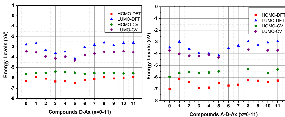
Figure 16. Comparison of frontier orbitals' energy levels obtained from cyclic voltammetry and DFT calculation.
