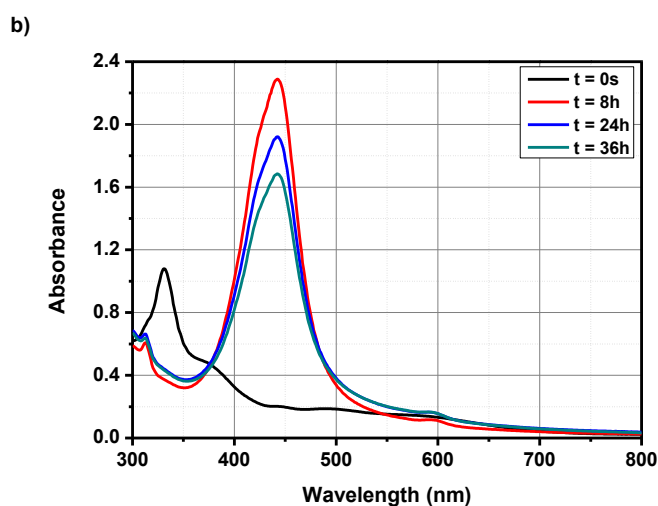
Figure 7. Evolution of the UV-visible absorption spectra of D-A1 and A-D-A1 in DMSO over time
