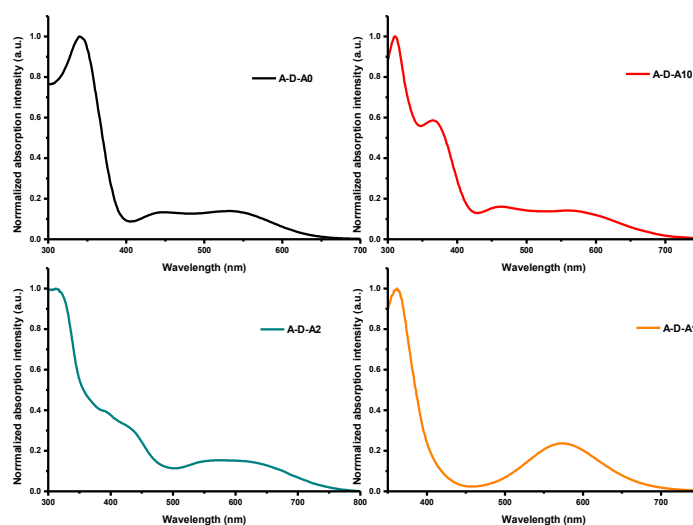
Figure 4. Normalized UV-visible absorption spectra of A-D-A triads A-D-A0 , A-D-A1 , A-D-A2 and A-D-A10 in chloroform.
