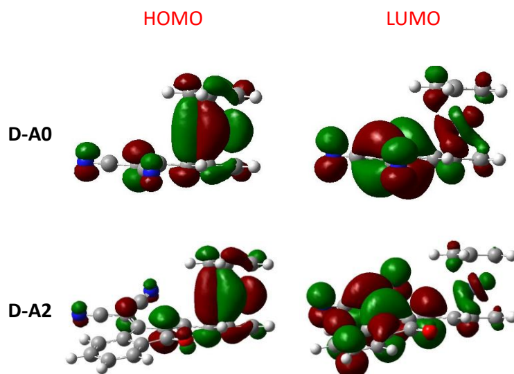
Figure 18. Contour plots of the electronic distribution of the HOMO and LUMO orbitals of D-A0 and D-A2.
