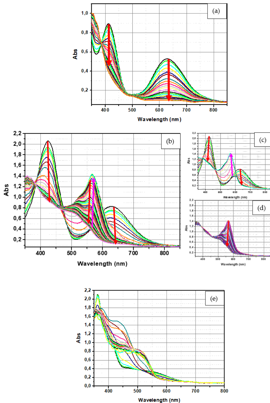
Figure 17. UV-Visible spectrum of (a) D-A2 , (b) full spectra for D-A4 (c) during the first minute for D-A4 , (d) during the last minute for D-A4 and (e) A-D-A11 in dichloromethane.
