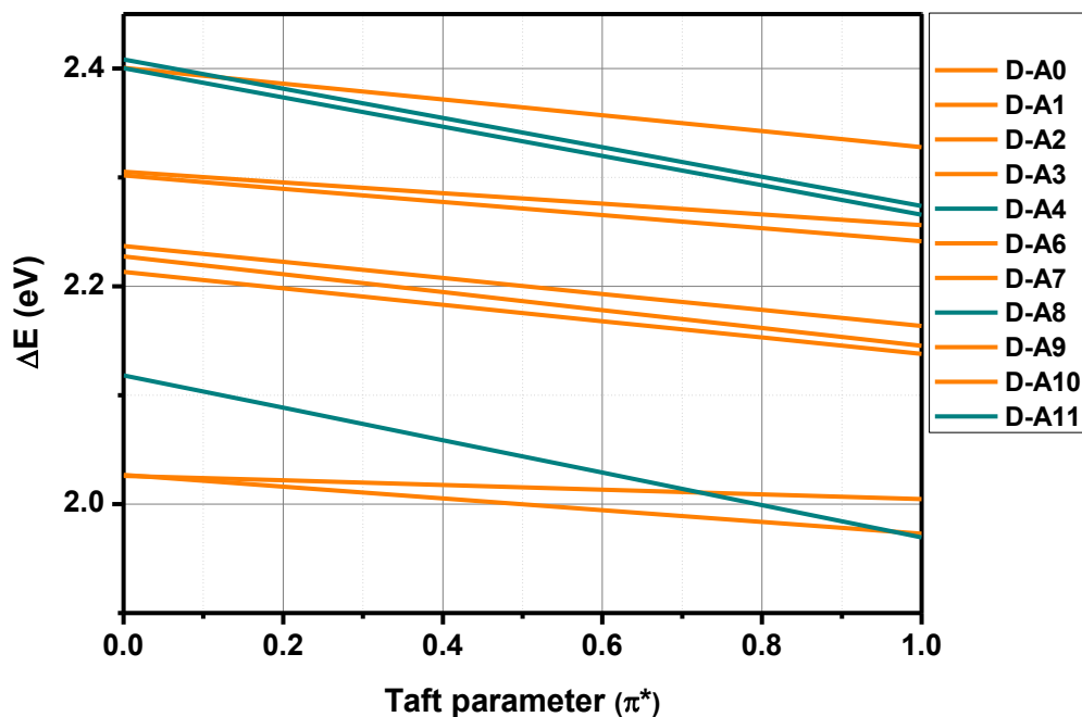
Figure 14. Variations of the HOMO-LUMO gaps with the Taft parameters.
