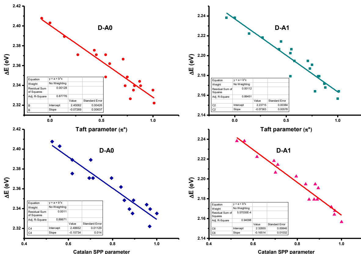
Figure 11. Linear correlations obtained for D-A0 and D-A1 using the Kamlet-Taft and the Catalan empirical scales.
