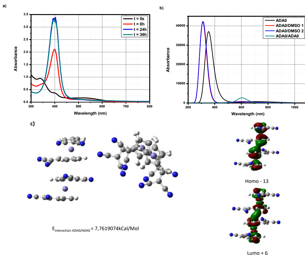
Figure 10. a) UV-visible absorption spectra of A-D-A0 over time in DMSO b) Theoretical UV-visible absorption spectra of A-D-A0 in DMSO and c) Geometrical optimization for A-D-A0 dimers and contour plots for HOMO-13 and LUMO+6.
