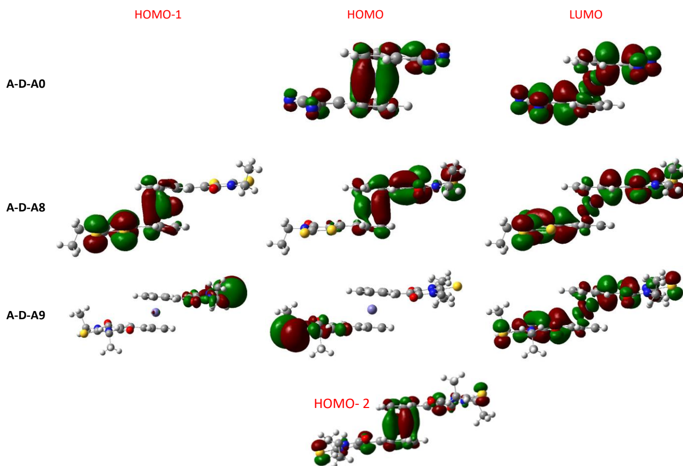
Figure 19. Contour plots of the electronic distribution of the HOMO and LUMO orbitals of A-D-A0 and A-D-A8 and A-D-A9
