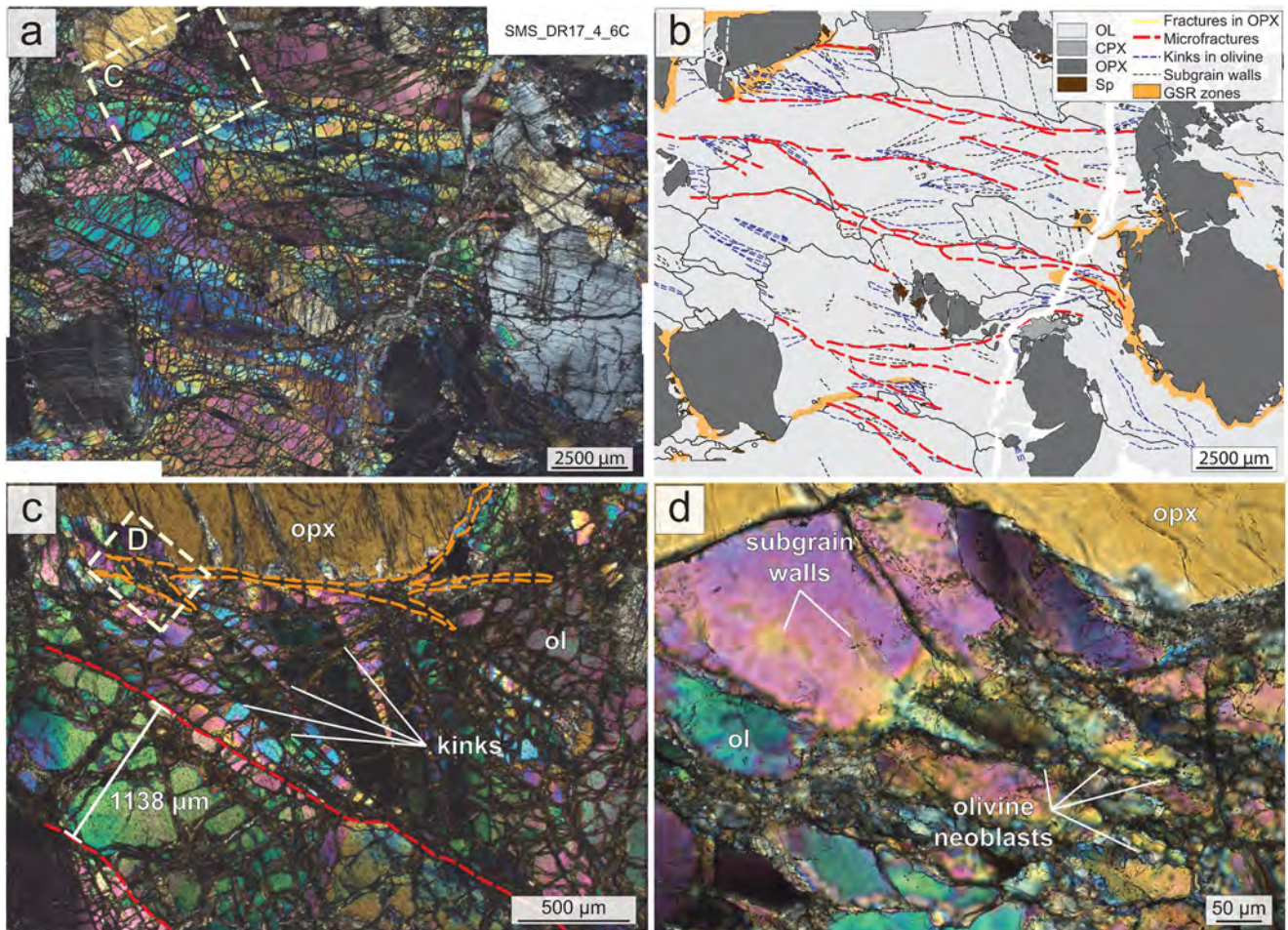
Figure 6. Microphotographs and associated sketch of kink bands, GSR zones and microfractures in olivine in textural type A2 samples. Sample SMS-DR17-4-6, thin section C, orthogonal to the thin section shown in Figure 5. (a) Crossed-nicols microphotograph and (b) structural interpretation (cracks and veins associated with serpentinization are not shown). Olivine is strongly deformed with kink bands, some of which are paralleled by microfractures. Kinked olivine displays marked undulose extinction and subgrain boundaries oblique to the kink bands. Kink bands in olivine share a preferred orientation at the thin section and sample scales. Microfractures follow olivine grain and subgrain boundaries. They branch into GSR zones next to orthopyroxene porphyroclasts. (c) Crossed-nicols microphotograph located in (a). Kink bands, some of which are paralleled by microfractures, form a horse-tail structure that branches into a larger microfracture (in red). A thin GSR zone (underlined by orange dashed line) develops next to the orthopyroxene porphyroclast. (d) Detail of (c). In the GSR zone, thin anastomosing domains of finely recrystallized olivine grains develop along the kink bands.
