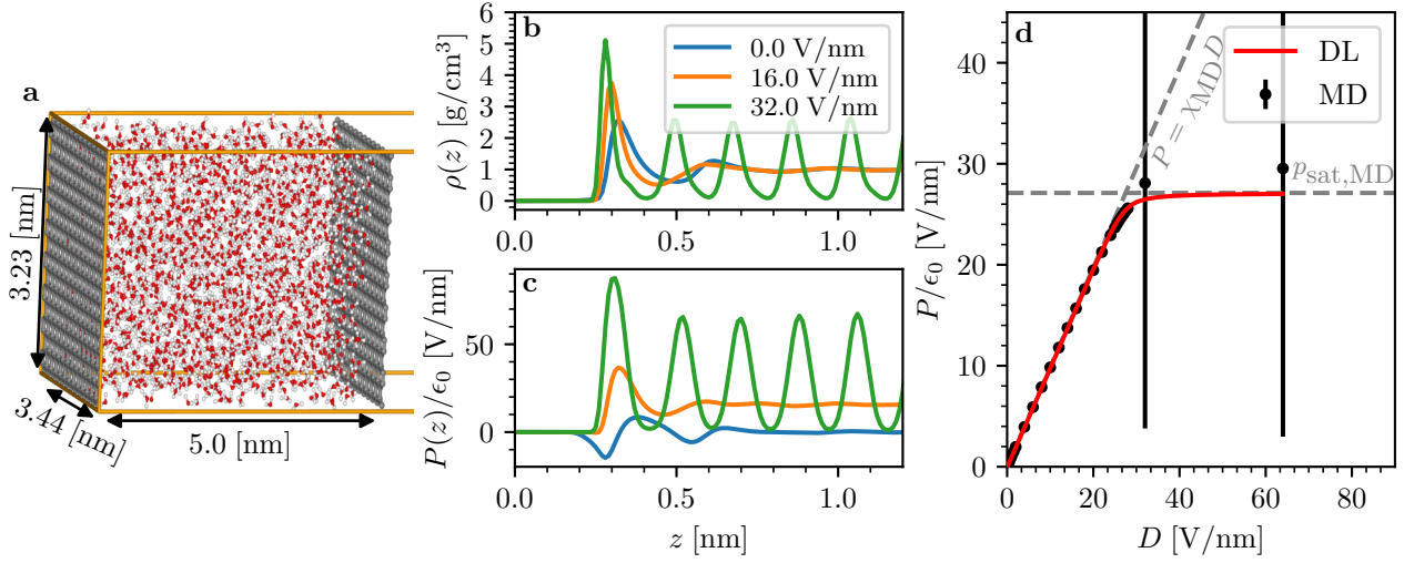
FIG. 3. Molecular dynamics simulations of SPC/E water under excitation field. a. Snapshot of the system composed of water molecules between two graphene sheets. Mass density (b.) and polarization (c.) for three different excitation fields D_0/\epsilon = 0 \text{ V.nm}^{-1} (blue plot), D_0/\epsilon = 16 \text{ V.nm}^{-1} (yellow plot), D_0/\epsilon = 32 \text{ V.nm}^{-1} (green plot). d. Polarization response as a function of the excitation field: MD simulations (black points); exact DL model (red plot); linear regime (dashed grey line), P = \chi_{\text{MD}}D_0 ; saturation polarization (horizontal dashed grey line) P = p_{\text{sat}} .
