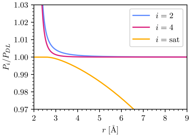
FIG. 5. Rescaled polarization response to a monovalent ion calculated for low and high fields regimes of the DL model. The rescaled linear polarization P_{\text{ion},2}/P_{\text{ion,DL}} (Eq. (18)) is plotted in blue, the rescaled fourth-order polarization P_{\text{ion},4}/P_{\text{ion,DL}} is plotted in pink and the rescaled saturated polarization P_{\text{ion,sat}}/P_{\text{ion,DL}} is plotted in yellow. The parameters used are given in Fig.(4).
