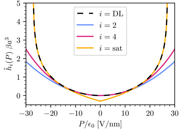
FIG. 4. Free energy density in the low- and high-field regime for the DL-model. The fourth-order expression \tilde{h}_{4,\text{DL}}(P) (Eq. (22), pink curve) and the large polarization expansion \tilde{h}_{\text{sat},\text{DL}}(P) (Eq. (24), yellow curve) of the dipolar free energy density are compared to the exact density \tilde{h}(P) (dashed black curve) and its harmonic expansion (blue curve). The cusp in P = 0 for \tilde{h}_{\text{sat},\text{DL}}(P) is outside of the validity zone of the expansion and has no physical meaning. The parameters used are obtained from SPC/E water simulations: p_0 = 9.62 \text{ D} , a = 0.51 \text{ nm} .
