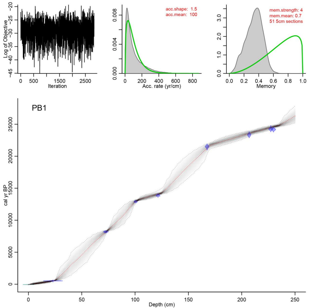
Figure 3. Age-depth model for Pearly Beach (PB1) using the Bacon software package (Blaauw and Christen, 2011). The blue areas represent the 2\sigma probability distributions of the calibrated ^{14}\text{C} ages, the grey-scales indicate all likely age-depth models, grey dotted lines show the 95% confidence intervals and the red dotted line shows the single 'best' model based on the median age for each depth.
