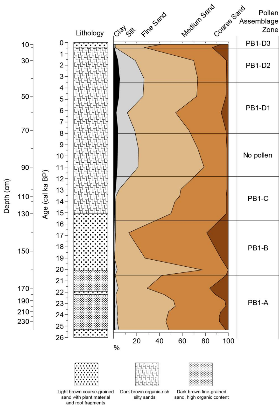
629 Figure 4: Pearly Beach 1 (PB1) particle size analysis data displayed as percentages of clay (0 – 2 µm), silt 630 (2 – 20 µm), fine sand (20 – 200 µm), medium sand (200 – 500 µm) and coarse sand (500 – 2000 µm) 631 plotted against interpolated age (cal kBP) and composite depth (cm) with pollen assemblage zones 632 indicated on the far right.
