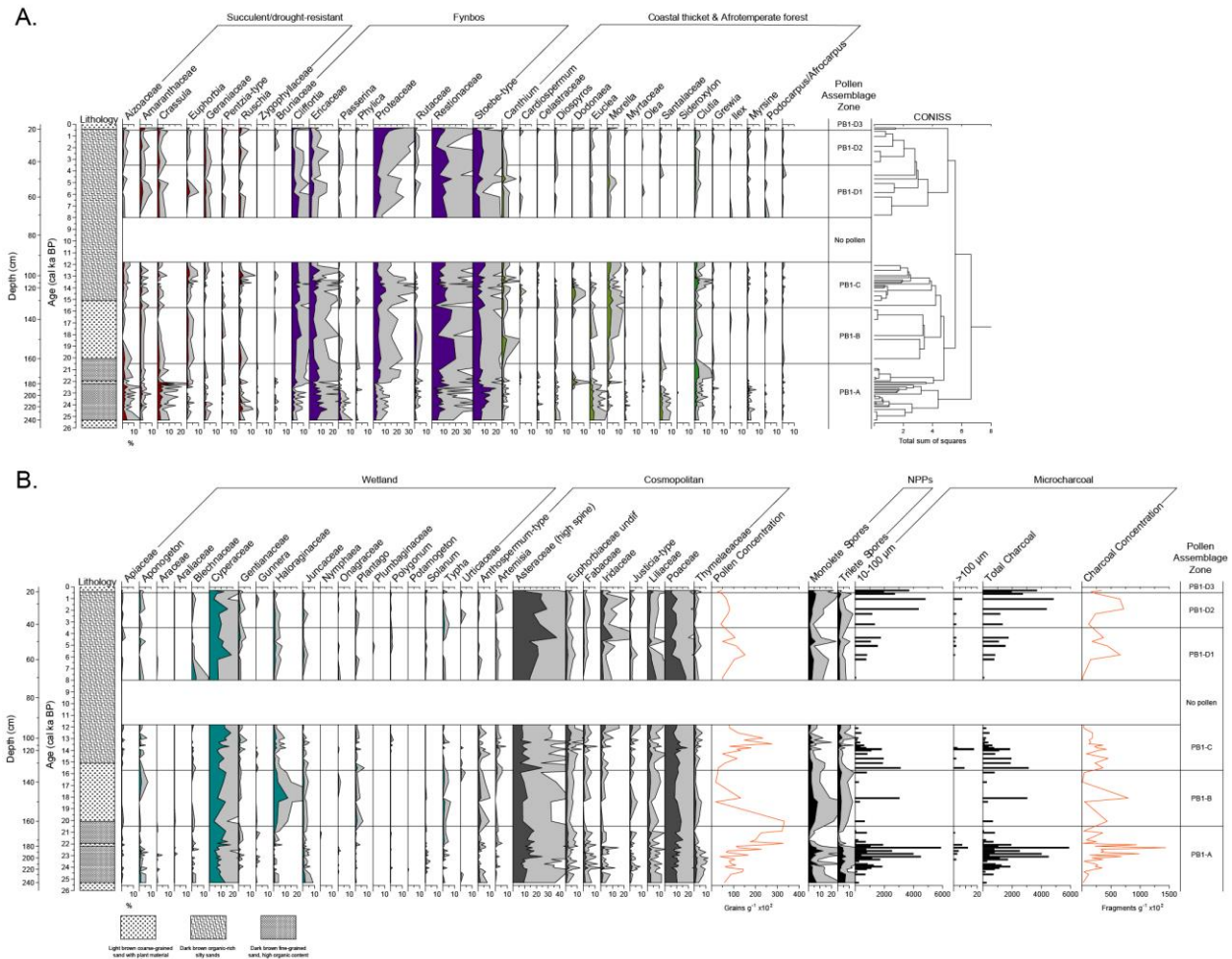
Figure 5 (A and B): Relative percentage pollen and microcharcoal diagrams for Pearly Beach (PB1). Taxa grouped according to general ecological affinities and are plotted against interpolated age (cal kBP) and composite depth (cm). Taxa included in the Cosmopolitan ecological grouping that represent less than 2% for any given level were excluded, the full dataset is presented in Appendix A. Exaggeration curves are 3x and zonation is based on the results of a CONISS analysis.
