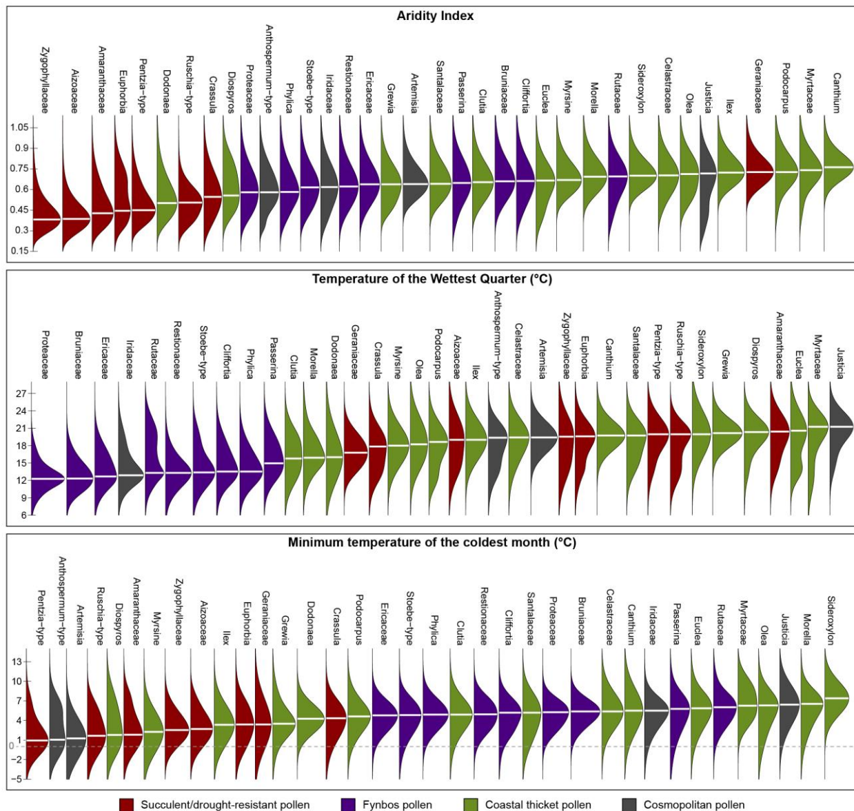
Figure 6: Probabilistic responses of the pollen taxa to three important regional climate determinants: Aridity index (Zomer et al., 2008; Trabucco and Zomer, 2019) and the temperature of the wettest quarter (used as a proxy for the temperature of the growing season) and the minimum temperature of the coldest month (Fick and Hijmans, 2017). These responses were calculated following the probability density function (pdf) approach of Chevalier et al. (2014) and using data from the SANBI database (SANBI, 2003), restricted to the plant species that currently live in the study area (defined here as a box between 17° and 29°E and between 32° and 35°S).
