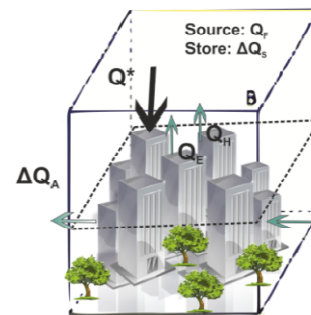
Fig.2. The energy balance of an urban building air volume (OKE, 1978).
