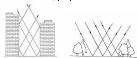
Fig.3. Illustration of radiative trapping (Griffiths, 1976)
