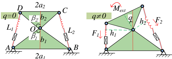
Figure 1: Geometry of a single segment of the mechanism.
