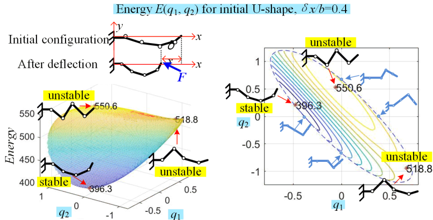
Figure 4: The energy function E(q_1, q_2) and manipulator equilibria for initial U-shape configuration (end-effector deflection \delta x/b=0.4 , \delta y=0 ; geometric parameters a/b=1.0 ; q_4>0 ).
