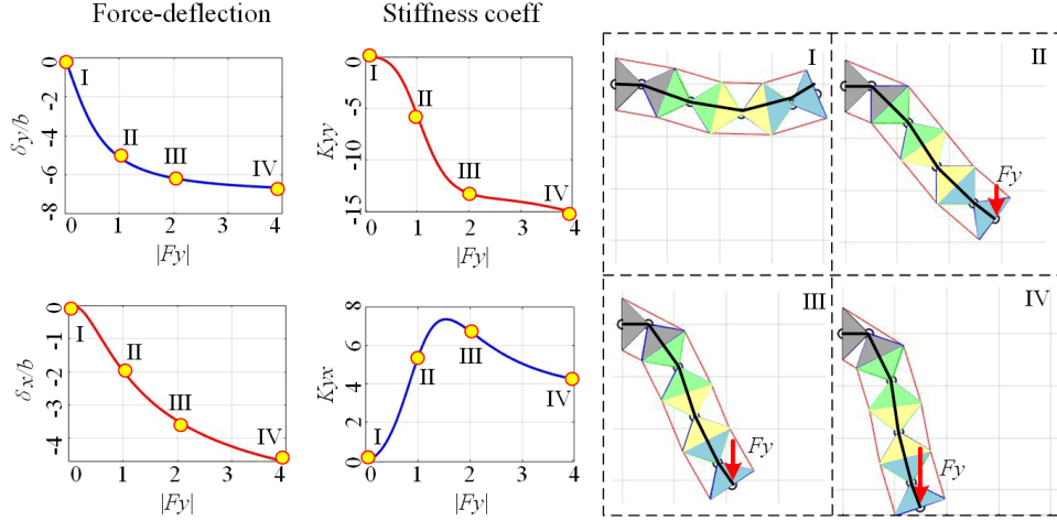
Figure 9: Stiffness coefficients under the F_x - and F_y -loading for initial U-shape configuration with (x_0, y_0) = (7.7b, 0) and geometric parameters a/b=1.0
