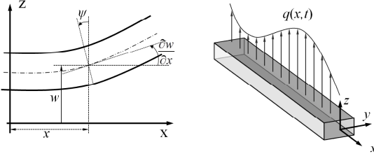
Figure 1: The coordinate system and kinematic parameters of the enriched Timoshenko beam model
