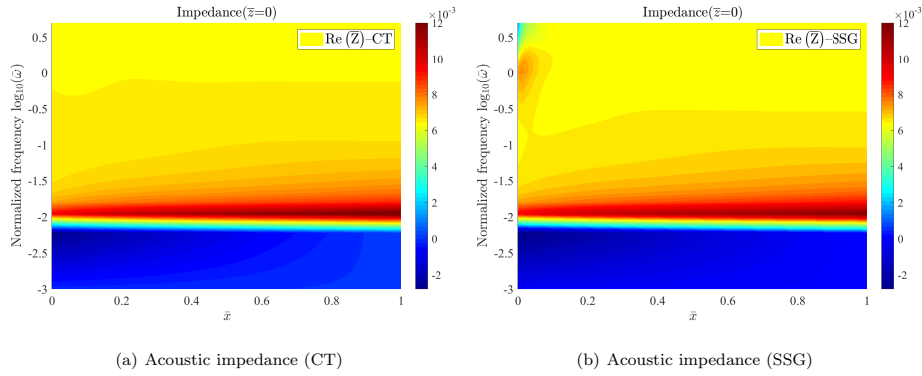
Figure 12: Acoustic radiation impedance
