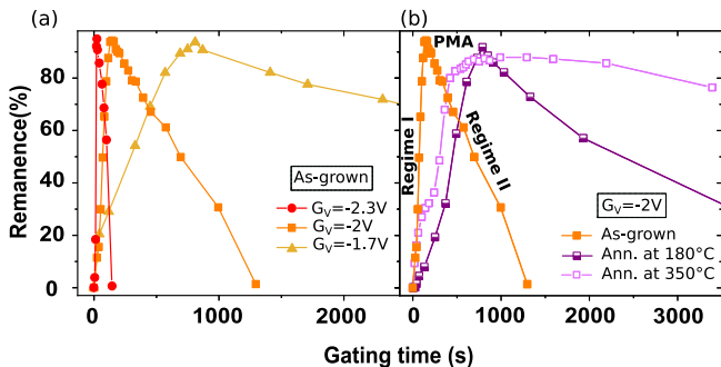
FIG. 3. Remanence as a function of gating time in (a) as-grown samples under G_V = -2.3 V (circles), G_V = -2 V (squares), and G_V = -1.7 V (triangles). (b) Samples annealed at 180 C (half open squares) and 350 C (open squares) under G_V = -2 V.
