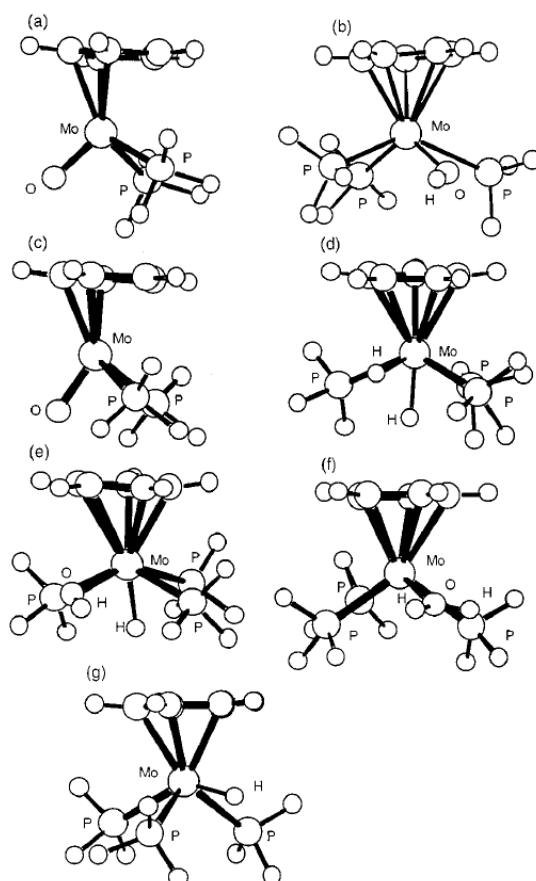
Fig. 6 Optimized geometries of (a) [CpMoO(PH 3 ) 2 ] + ; (b) [CpMo(OH)(PH 3 ) 3 ] + ; (c) CpMo(OH)(PH 3 ) 2 ( S = 1/2); (d) [CpMoH 2 (PH 3 ) 3 ] + ; (e) [CpMoH(OH)(PH 3 ) 3 ] + ; (f) [CpMo(PH 3 ) 3 (H 2 O)] + ; (g) [CpMoH(PH 3 ) 3 ] + .
