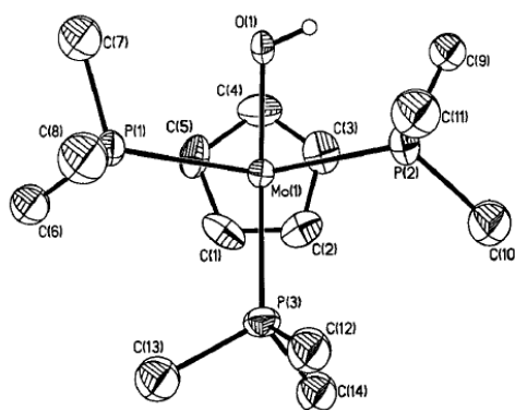
Fig. 3 A top view of the [\text{CpMo}(\text{OH})(\text{PMe}_3)_3]^+ cation in the structure of [\text{CpMo}(\text{OH})_{0.79}\text{Cl}_{0.21}(\text{PMe}_3)_3]^+\text{BF}_4^- . Ellipsoids are drawn at the 30% probability level.
