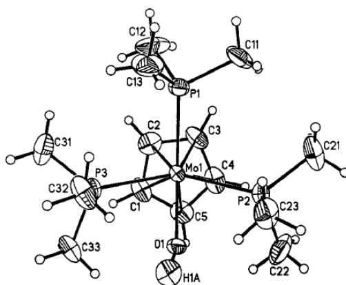
Fig. 2 A top view of the [\text{CpMo}(\text{OH})(\text{PMe}_3)_3]^+ cation in compound 2 . Only the major orientation of the disordered \text{PMe}_3 ligand (P1 donor atom) is shown for clarity.
