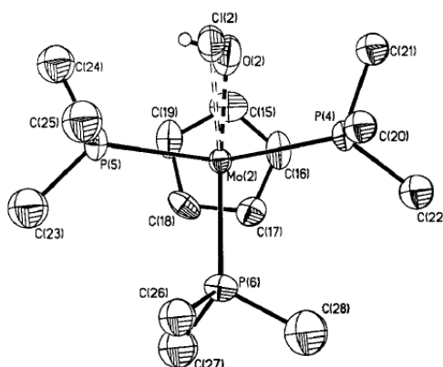
Fig. 5 A view of the [CpMo(O)(PMe 3 ) 2 ] + ion in compound 3 . Ellipsoids are drawn at the 30% probability level.
