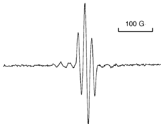
Fig. 1 Room temperature EPR spectrum of a solution of 4 in \text{CD}_3\text{COCD}_3 .
