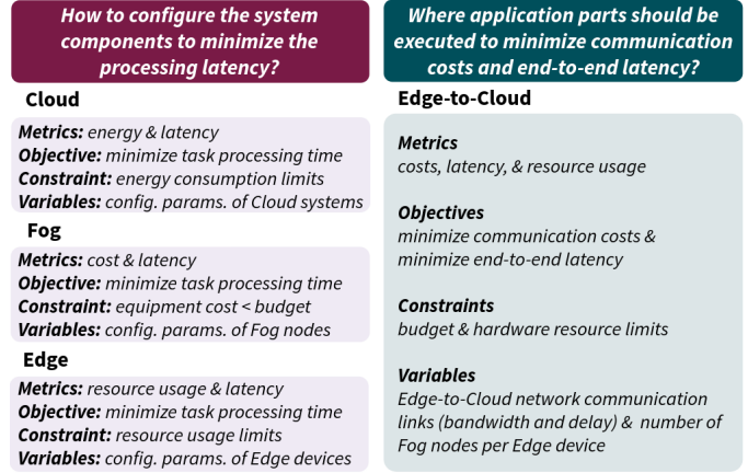
Fig. 4: Edge-to-Cloud Continuum optimization problems.
