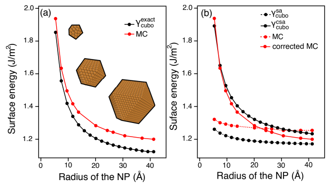
FIG. 1. Calculated surface energies for cuboctahedron Cu NPs as a function of size based on an (a) exact surface S(k) and (b) a spherical (sa) approximation (csa) as well as corrected spherical approximation (csa). Both figures present analytical and MC results.
