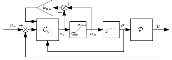
Figure 7: Anti-windup action.
