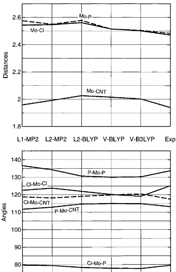
Figure 5 Optimized distances (in Å) and bond angles (in degrees) for the ^2A' \text{CpMoCl}_2(\text{PH}_3)_2 system with symmetry-equivalent \text{PH}_3 ligands ( II ) and comparison with the experiment ( \text{CpMoCl}_2(\text{PMe}_3)_2 , Ref. 3b). CNT is the centroid of the Cp ring.
