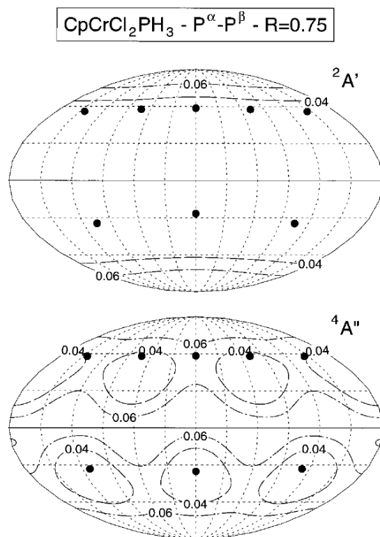
Figure 2 Contour plot of the excess electron spin density (au) obtained using the V-BLYP Kohn-Sham orbitals at a radial distance of 0.75 Å from the metal center in the ^2A' (top) and ^4A'' (bottom) states of \text{CpCrCl}_2\text{PH}_3 . Other drawing parameters are as in Figure 1.
