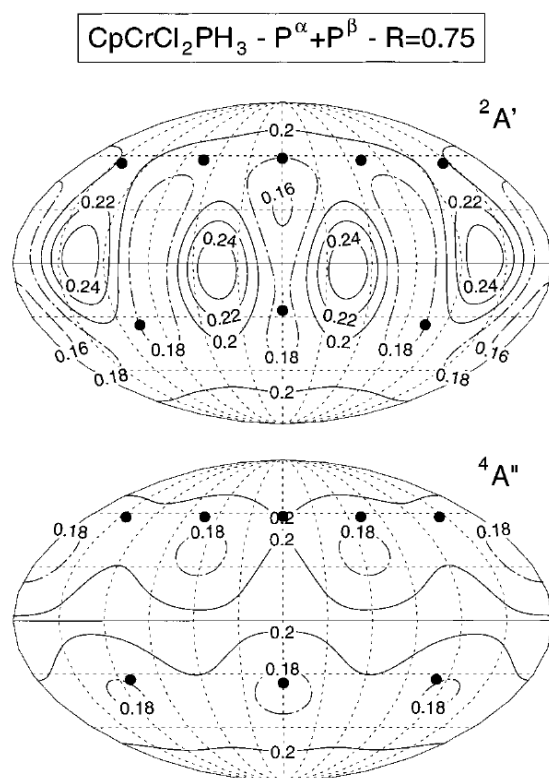
Figure 1 Contour plot of the total electron density (au) obtained using the V-BLYP Kohn-Sham orbitals at a radial distance of 0.75 Å from the metal center in the 2 A' (top) and 4 A'' (bottom) states of CpCrCl 2 PH 3 . The dots represent the projected image of the ligand atoms on the surface of the sphere (H atoms neglected). The “parallels” are traced at intervals of 30° for the polar angle θ (from 0°, top, to 180°, bottom); the “meridians” indicate the azimuthal angle φ at intervals of 30°
