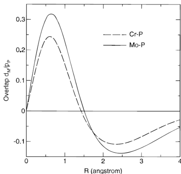
Figure 7 Overlap between the nd_{x^2-y^2} ( n = 3 for M = \text{Cr} , n = 4 for M = \text{Mo} ) and the 3p orbital of phosphorus along the M-P axis for the CpMCl 2 PH 3 4 A” system. ROSCF calculations on basis LanL2DZ.
