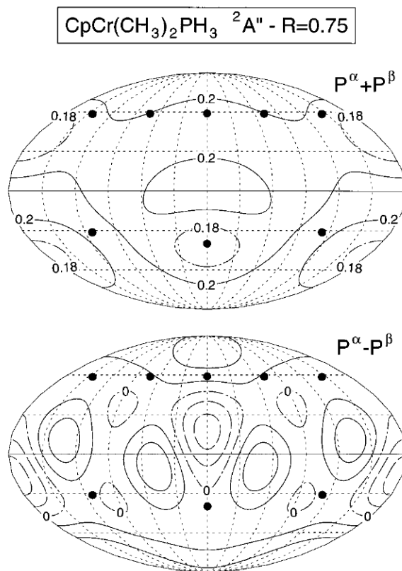
Figure 3 Contour plot of the total (top) and excess (bottom) electron spin density (au) obtained using the V-BLYP Kohn-Sham orbitals at a radial distance of 0.75 Å from the metal center in the ^2A'' state of \text{CpCr}(\text{CH}_3)_2\text{PH}_3 . In the lower part of the figure, only the zero-density contour lines are labeled. Dashed lines are for negative ( \beta spin excess), full lines for positive ( \alpha spin excess) density. Contour lines are drawn at 0.03 au intervals. Other drawing parameters are as in Figure 1.
