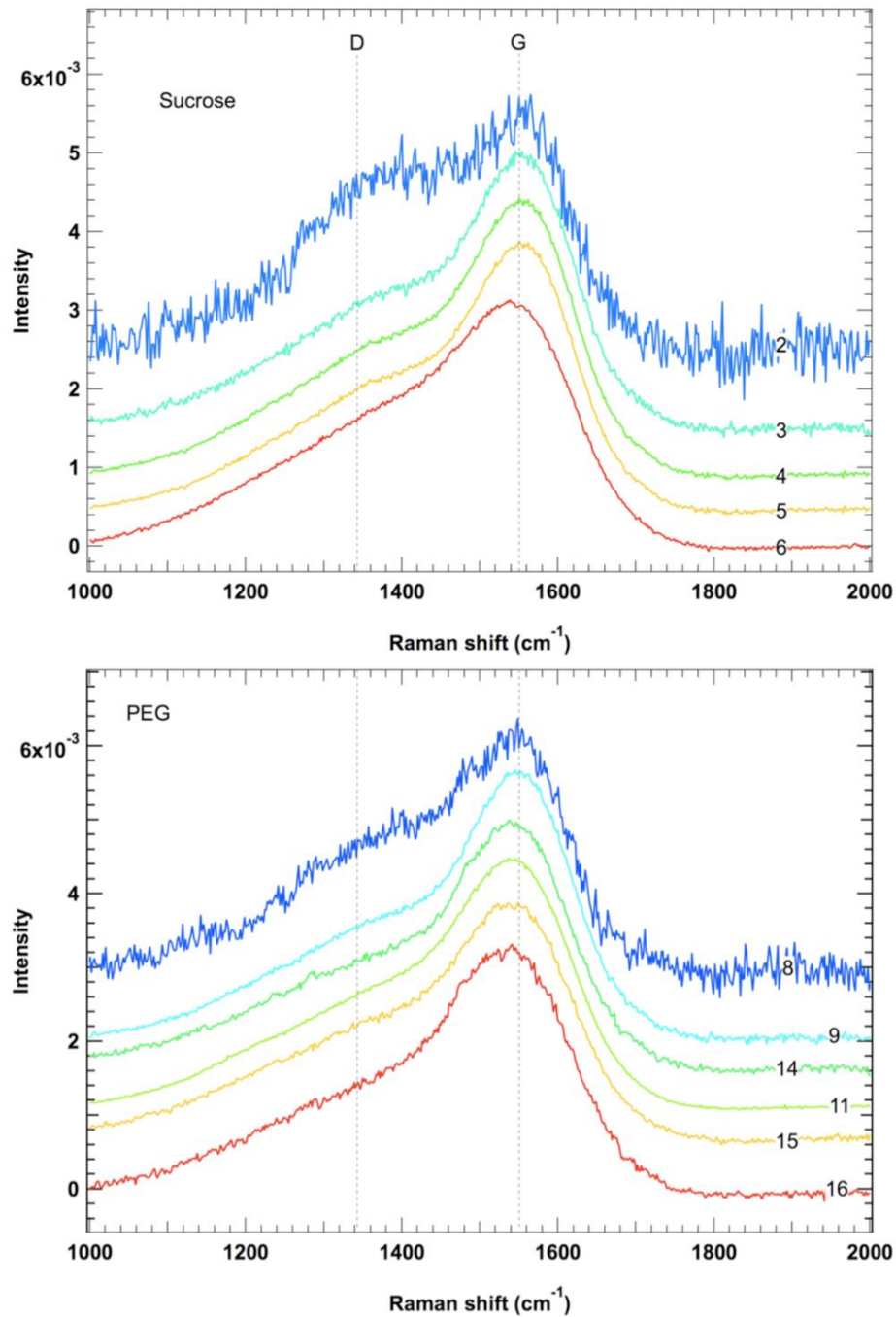
Figure A4: Visible Raman spectra ( \lambda=532 \text{ nm} ) in the range 1000 \text{ cm}^{-1} , 2000 \text{ cm}^{-1} of sucrose and PEG irradiated with 170 keV Neon and 40 keV Carbon. For each precursor, the highest spectrum (blue) is obtained at the nuclear dose from which the D and G bands appear, and then downwards, those obtained for increasing doses. The numbers refer to those indicated in Table 1. Spectra are vertically shifted for the sake of clarity.
