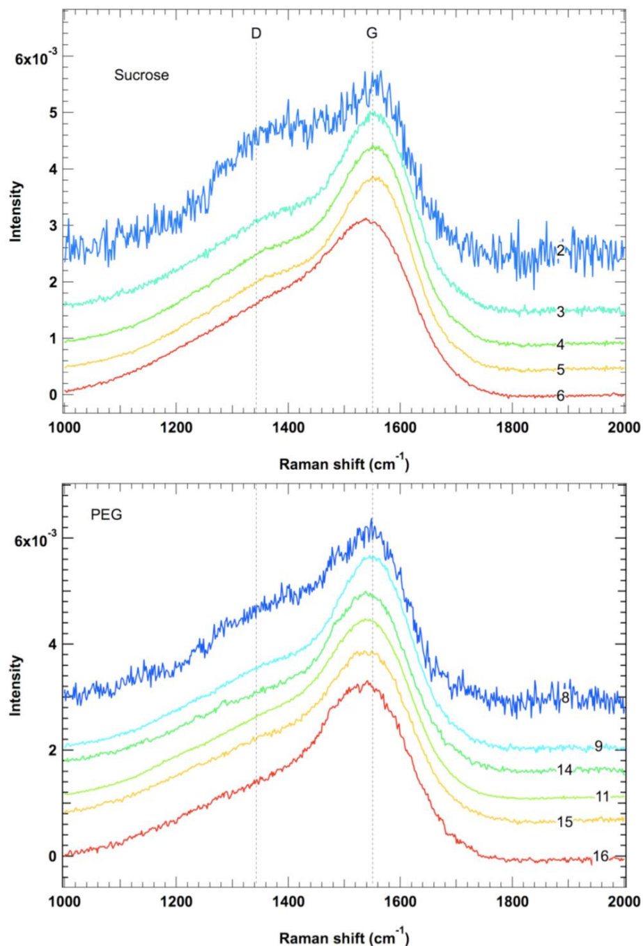
Figure A4: Visible Raman spectra ( \lambda=532 nm) in the range 1000 \text{cm}^{-1} , 2000 \text{cm}^{-1} of sucrose and PEG irradiated with 170 keV Neon and 40 keV Carbon. For each precursor, the highest spectrum (blue) is obtained at the nuclear dose from which the D and G bands appear, and then downwards, those obtained for increasing doses. The numbers refer to those indicated in Table 1. Spectra are vertically shifted for the sake of clarity.
