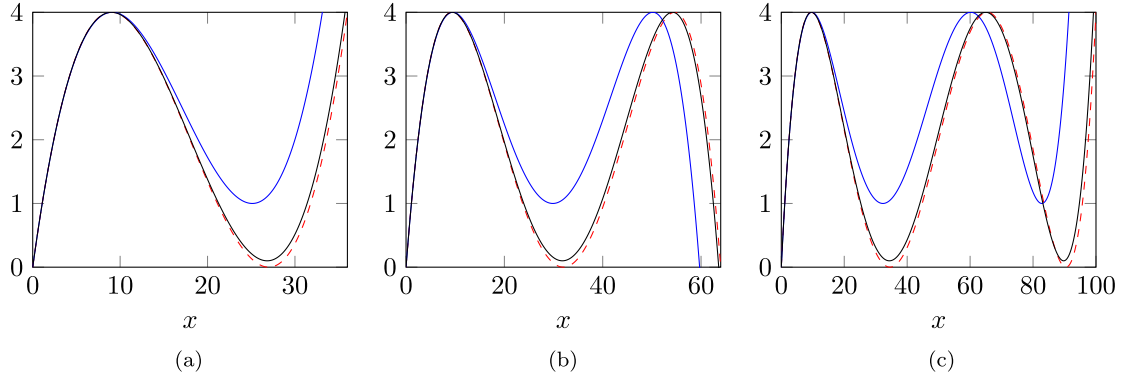
FIGURE 3. Plain line: Representation of x\mathcal{P}_{p,\ell}^\epsilon(x) for different values of \ell and for \epsilon = 0.1 (in black) or \epsilon = 1 (in blue). Dashed line: Representation of x\tilde{\mathcal{P}}_{p,\ell}(x) for different values of \ell . (a) \ell = 2 . (b) \ell = 3 . (c) \ell = 4 .
