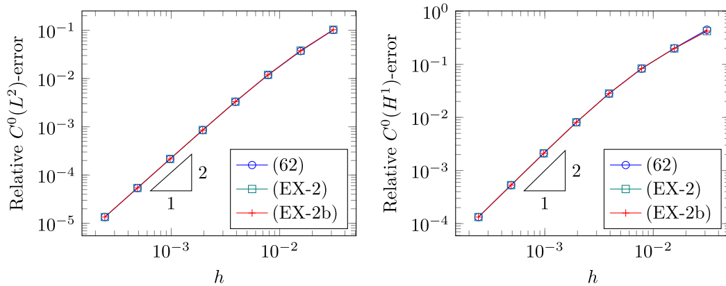
FIGURE 10. Space-time convergence plots for the LTS explicit scheme. The analytical solution is a propagating pulse.
