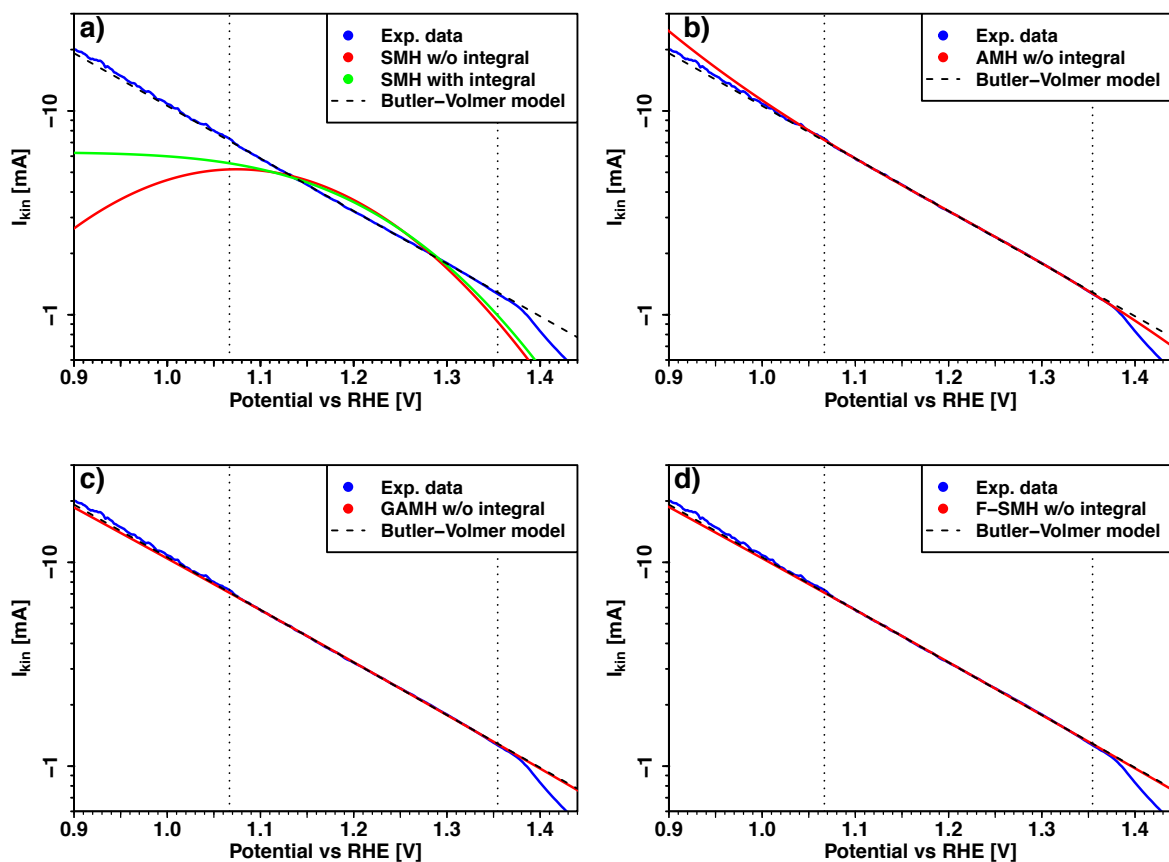
Fig. 4: Fits of SMH (a), AMH (b), GAMH (c), and Frumkin-SMH (d) models to our experimentally determined kinetic current of the Ce(IV) reduction on \text{Au}_{poly} . The dashed line shows the linear Tafel fit with the Butler-Volmer model.
