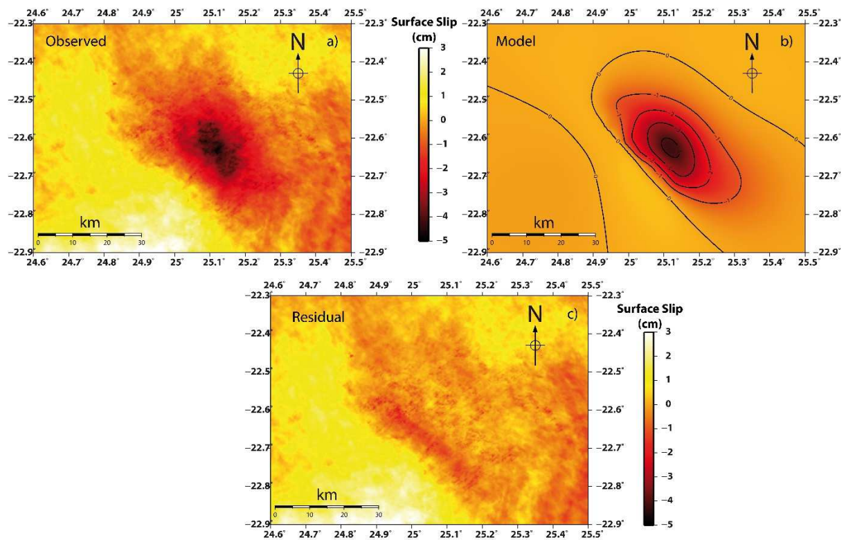
Figure 12 a) Unwrapped SAR data interferogram with surface slip distribution. b) Modelling of surface deformation from the inversion of InSAR data. c) Residual of InSAR results versus model.
