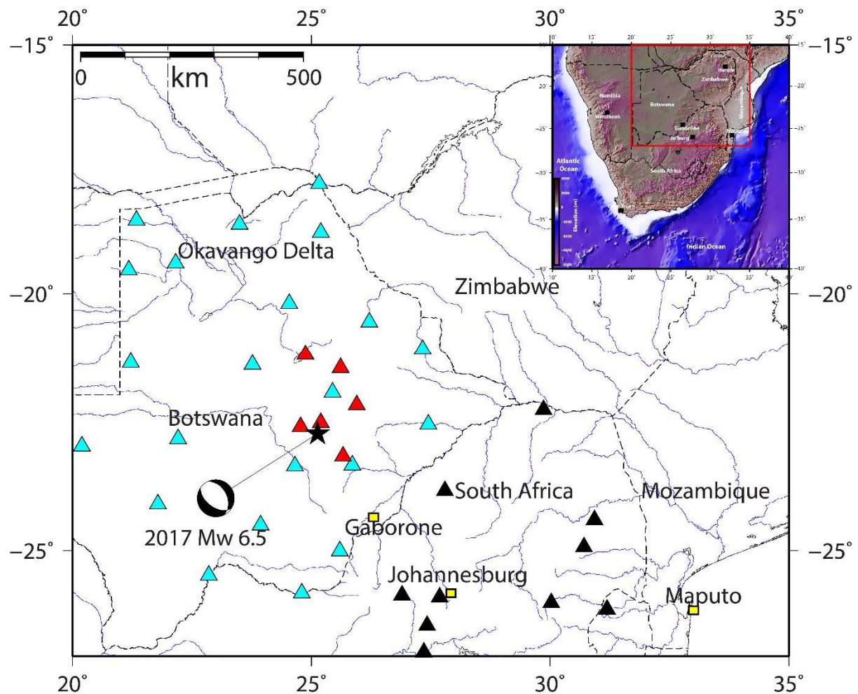
Figure 3. Seismic stations which recorded the mainshock (black star) and aftershocks. Focal mechanism is from Harvard CMT. The seismic stations in cyan triangles are managed by
