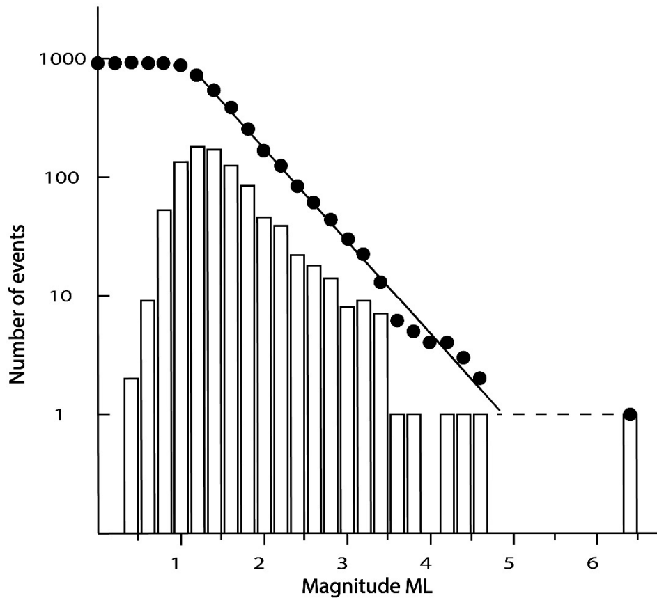
Figure 6. b) Gutenberg-Richter relation \text{Log } N = 3.8 - 0.78M_L as applied to the 2017 earthquake sequence.
