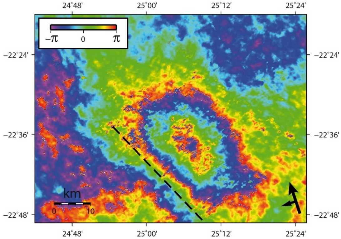
Figure 11. Fringes and lobes of interferogram of the 3 rd of April 2017 Botswana earthquake.
