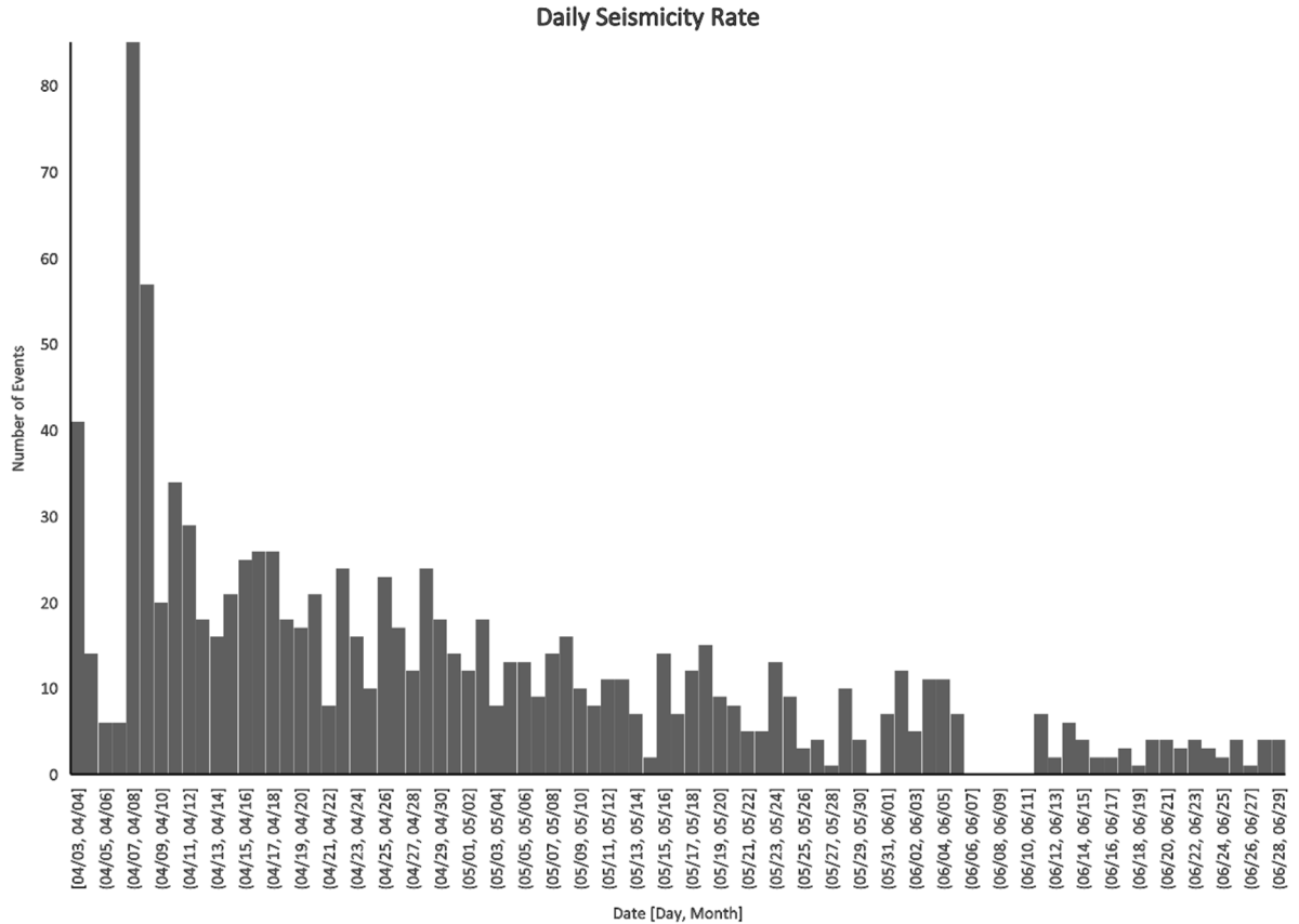
Figure 4. Daily number of seismicity recorded from the 3 rd of April to the 29 th of June 2017.
