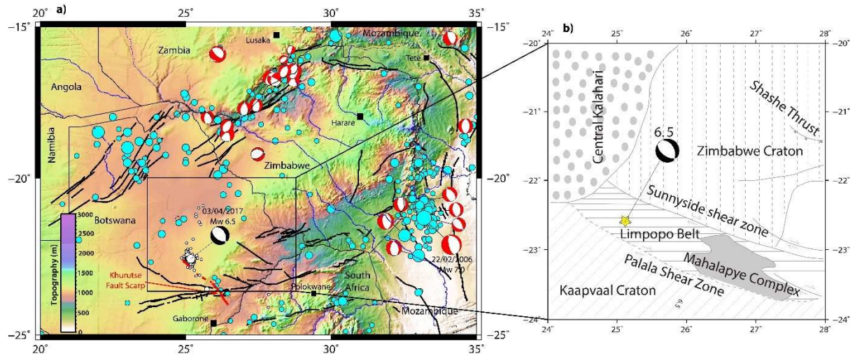
Figure 2. a) Seismotectonic framework excerpt of the Seismotectonic Map of Africa (modified from Meghraoui et al. , 2016) with focal mechanism (CMT-Harvard) of the 2017 Moiyabana mainshock. The red line is the inferred Khurutse fault scarp, cyan circles are background seismicity with magnitude 4.5 \leq M \leq 7.5 ; b) Structural geology background of the 2017 earthquake area (modified from Brown et al. , 2008). The mainshock is indicated by a yellow star.
