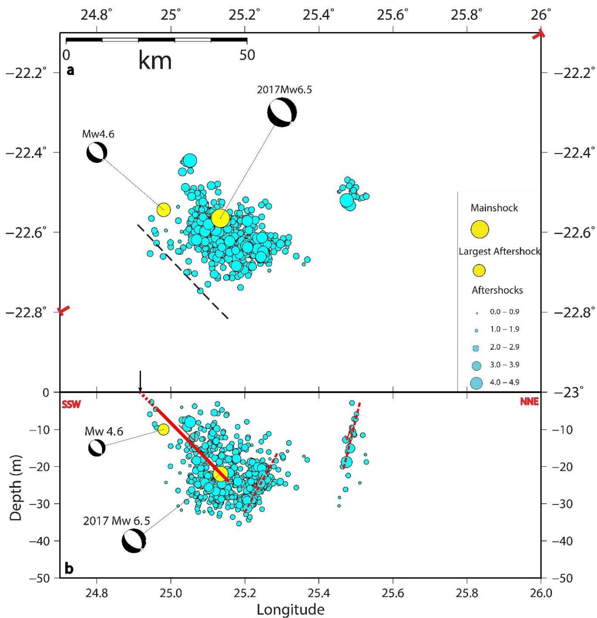
279 Figure 7. a) Spatial distribution of aftershock locations obtained after relocation. Focal 280 mechanism solutions of the mainshock and main aftershock are from CMT Harvard. The 281 dashed line is the coseismic rupture tip inferred from the aftershocks at depth (Fig. 7b) and 282 the analysis of InSAR fringes of coseismic surface deformation (see section on InSAR 283 analysis). b) Aftershock sequence cross-section, as indicated by the T-symbols in Fig. 7(a), 284 after relocation. Focal Red lines are the blind coseismic ruptures inferred from the
