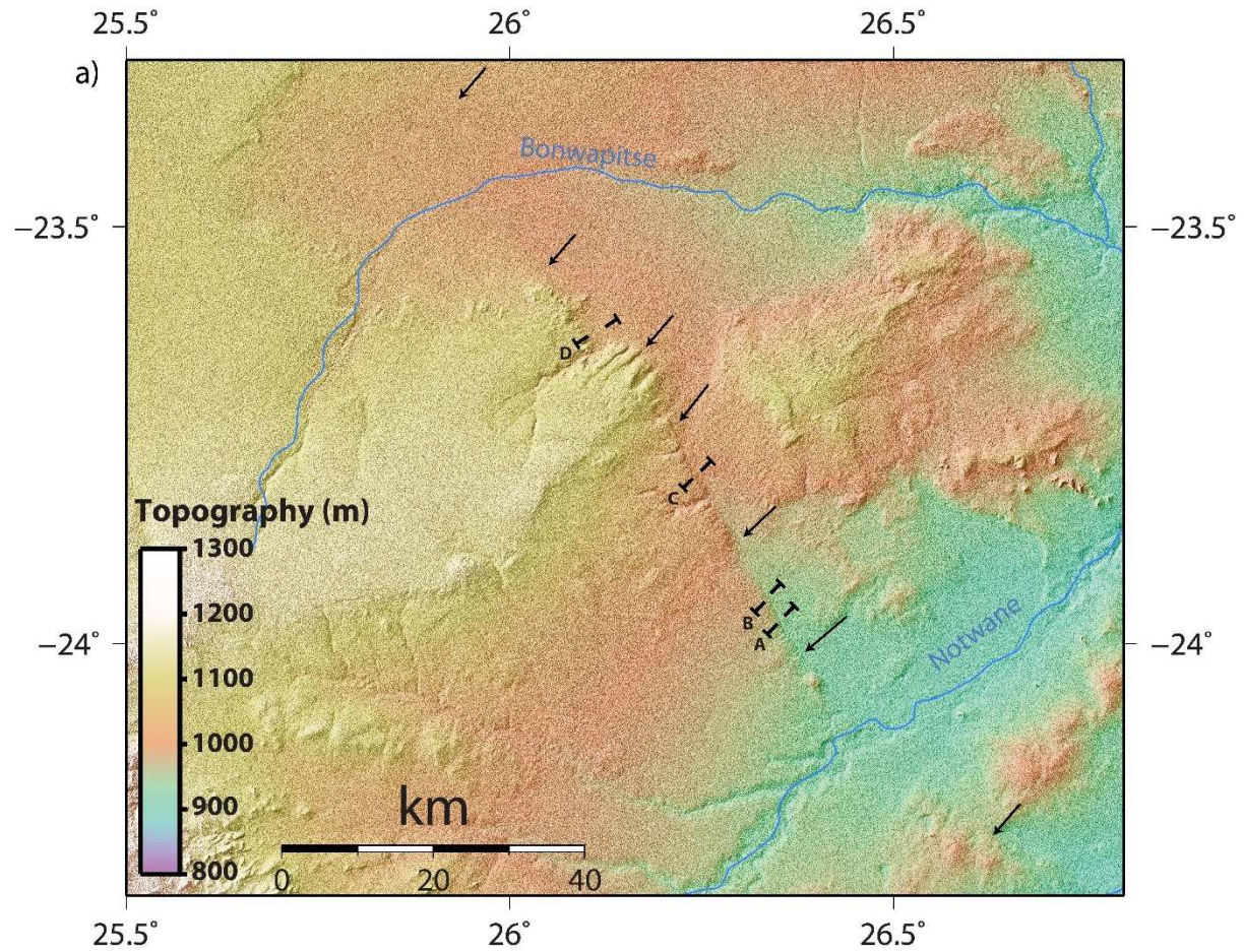
Figure 17. a) Detail of the Khurutse fault scarps (arrows, see also arrows in Fig. 15) with location of the cross-section profiles of Fig. 17(b) denoted A to D (background topography from SRTM 1" data).
