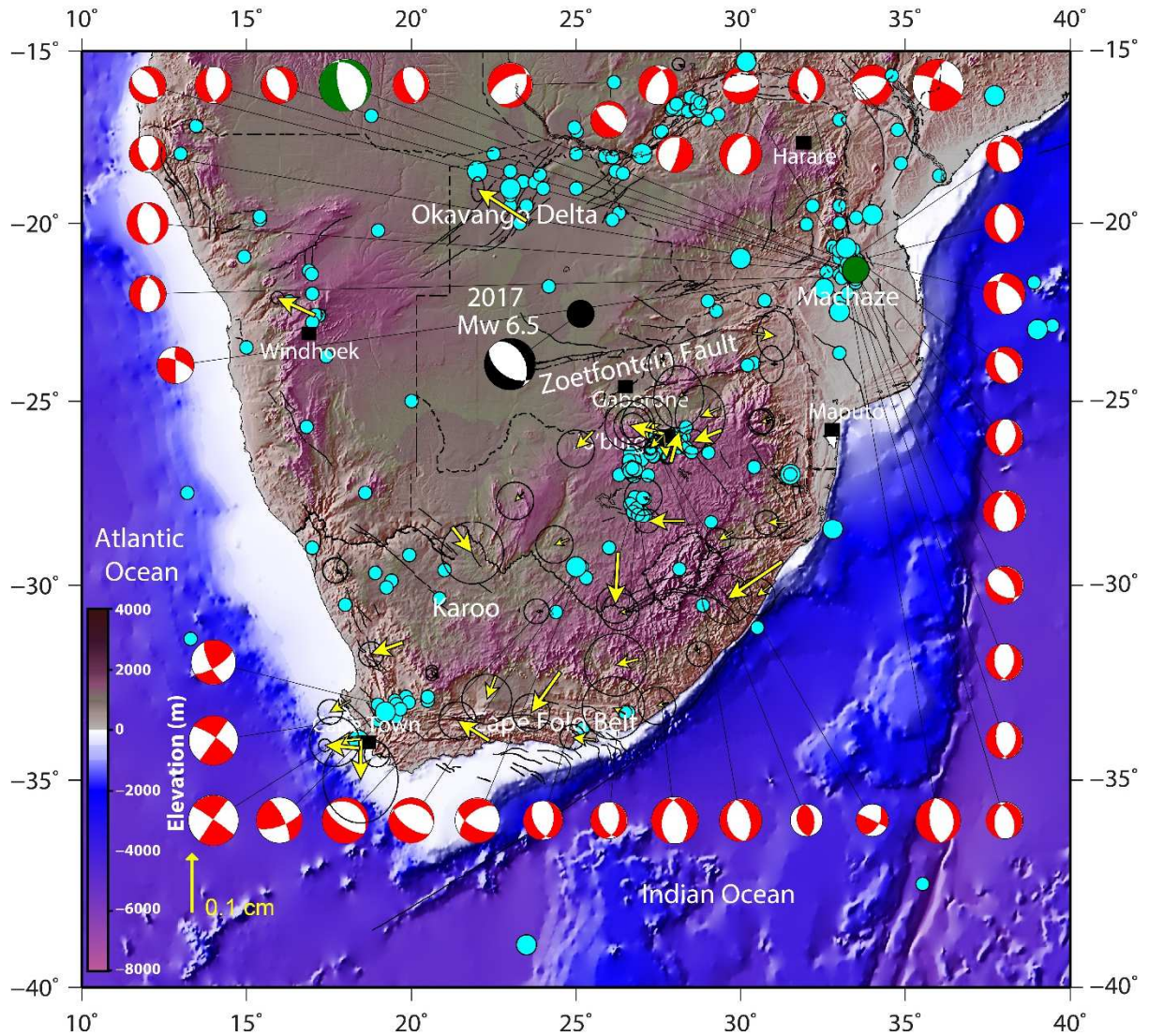
Figure 1: Seismotectonic background of southern Africa (light blue circles and red and white CMT focal mechanism solutions (SM1)), as updated from Meghraoui et al., (2016). Black circle is the location of the 3 April 2017 earthquake and its focal mechanism solution (black and white, CMT-Harvard, https://www.globalcmt.org/CMTsearch.html ). The green and white focal mechanism is of the 23 February 2006 Machaze earthquake (Mw 7.0, Mozambique, green circle). GPS velocities (Nubia fixed, yellow arrow with 1\sigma error ellipse) are from Saria et al. (2014).
