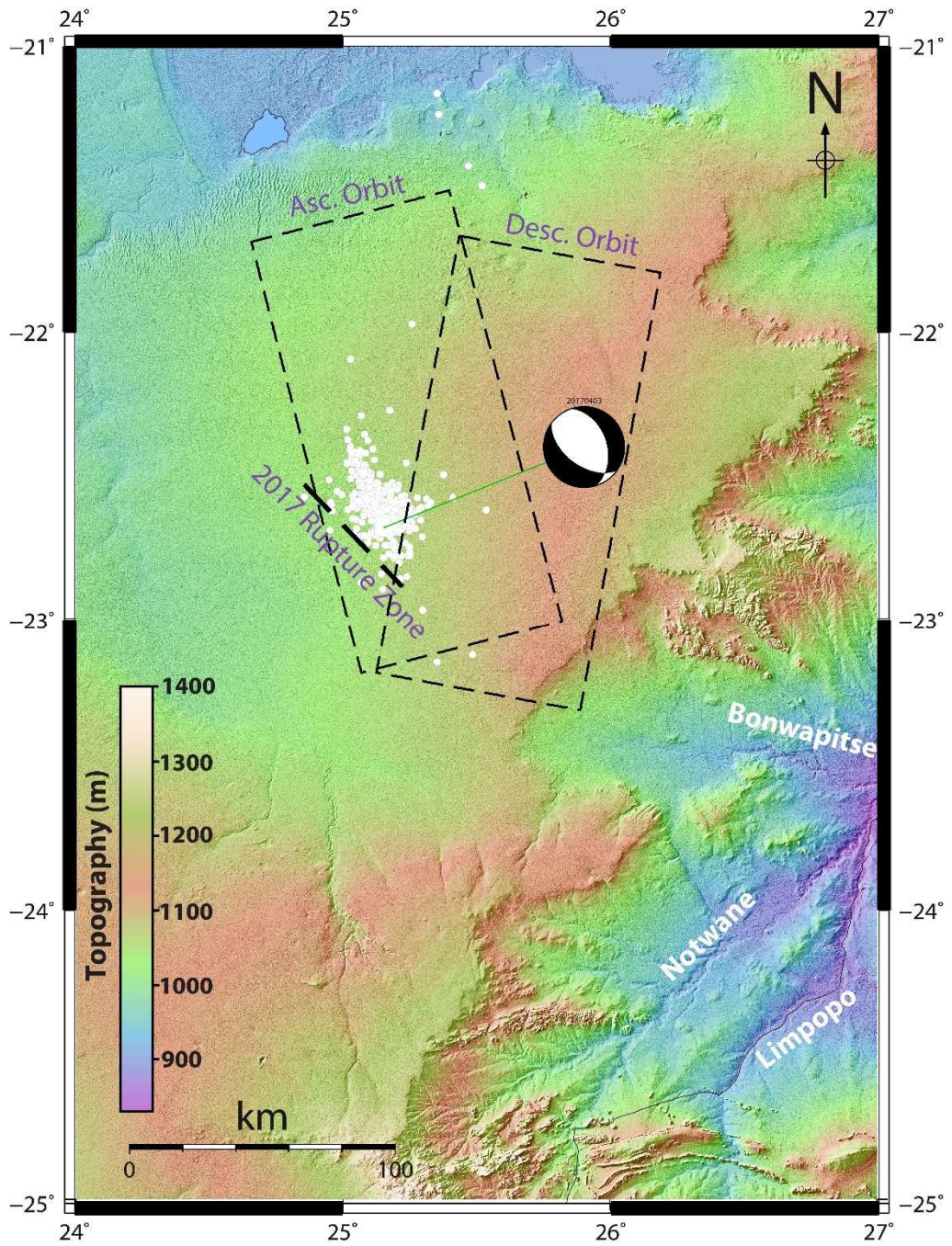
Figure 10. Frame of ascending and descending tracks of Sentinel-ESA-SAR images crossing the 2017 earthquake area. We observe that only the ascending track covers the whole 2017 earthquake area. Thick dashed line is the inferred 2017 Moiyabana earthquake rupture zone and small white circles show aftershock distribution. Focal mechanism of mainshock is from Harvard CMT. Background topography is from SRTM1'.
