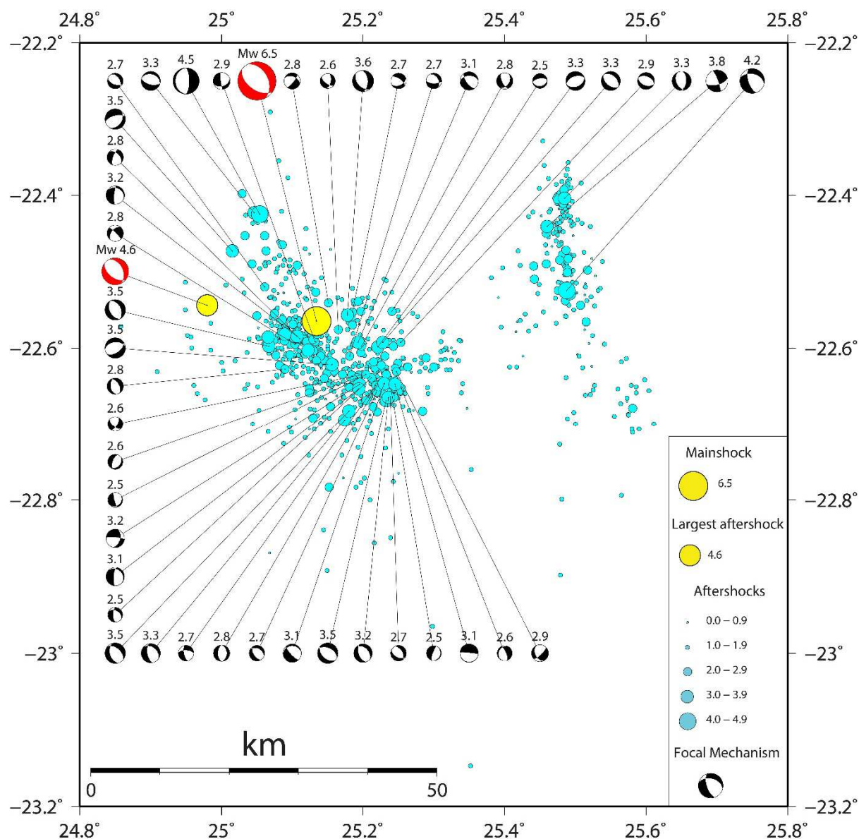
Figure 8. Focal mechanism solutions of 46 selected seismic events (see also Table SM4).
