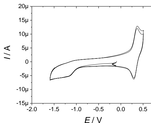
Figure 2 Cyclic voltammogram curve [Eu(L_2)]^{3+} in 0.5 mM CH_3CN solution containing 0.1 M TBAP. Scan rate, 0.1 V s^{-1} , T = 298 K, carbon electrode.
