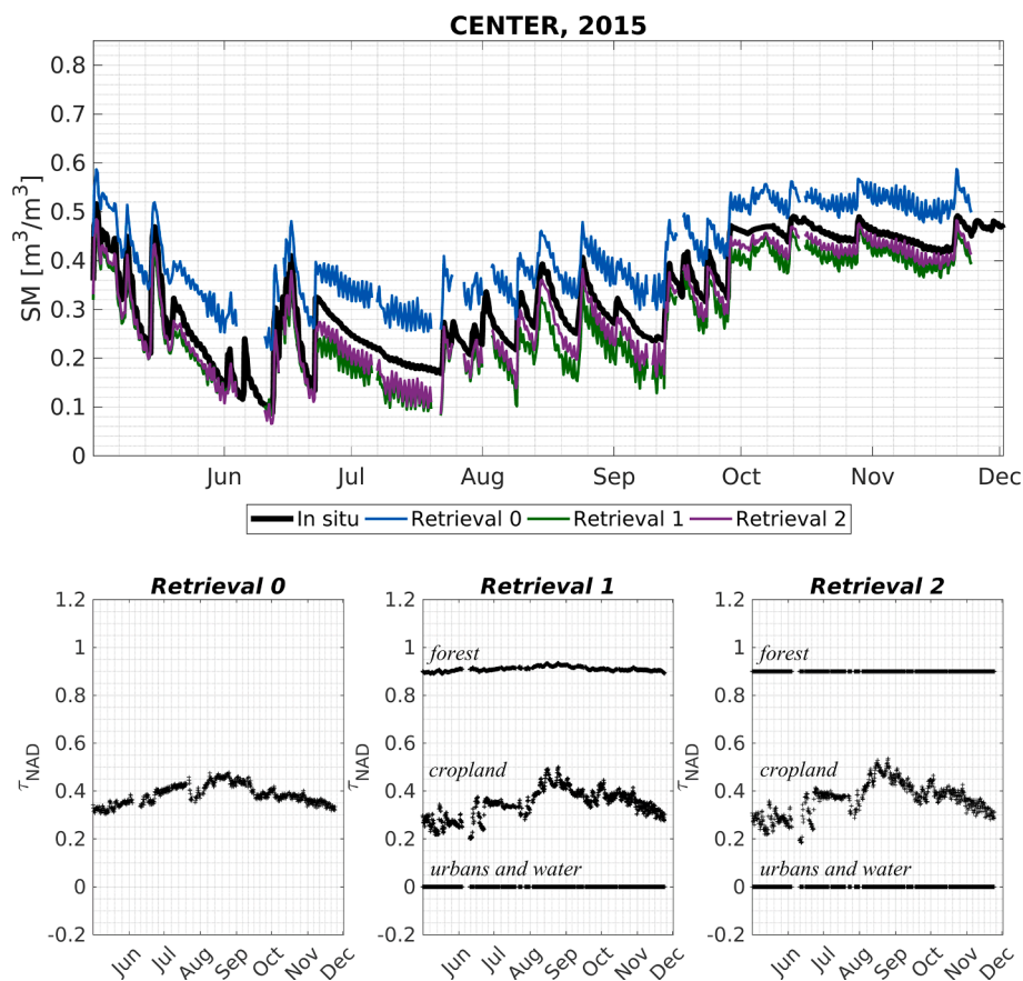
Fig. 6. Derived SM (top) and VOD (bottom) for retrievals V0, V1 and V2 over the CENTER scene.
