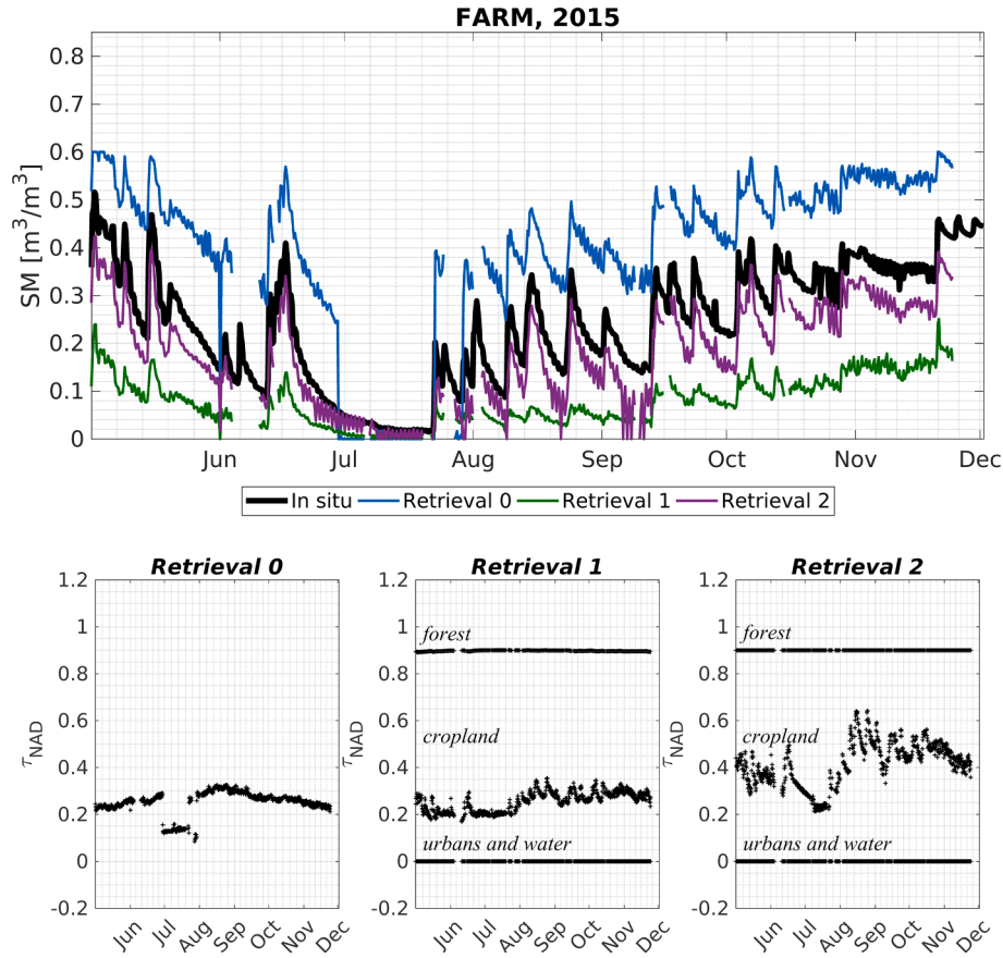
Fig. 7. Derived SM (top) and VOD (bottom) for retrievals V0, V1 and V2 over the FARM scene.
