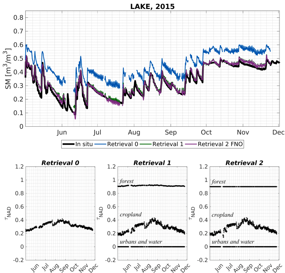
Fig. 5. Derived SM (top) and VOD (bottom) for retrievals V0, V1 and V2 over the LAKE scene.
