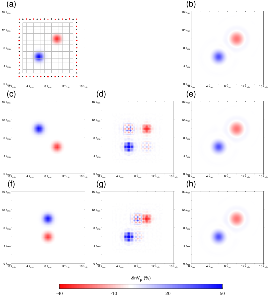
Figure 2. Smooth elastic FWI tests. (a) P wave velocities ( V_P ) for the target model ; (b) homogenized target model nearest isotropic P -wave velocity V_P^{\text{iso}} ; (c) and (f) two starting models V_P ; (d) and (g) raw inverted models V_P^{\text{iso}} for the starting models (c) and (f) respectively; (e) and (h) homogenized inverted models V_P^{\text{iso}} for the starting models (c) and (f) respectively; For each panel, only V_P is represented, but the other mechanical properties have the same shape. In (a) the red stars represent the position of the sources and the black triangles represent the position of the receivers. The black square is the area where the model parameters are inverted and the inside mesh is the inversion mesh.
