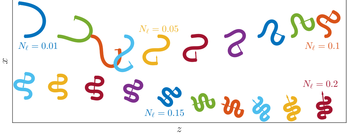
Figure 10: Dimensionless deformed shape of the beam glued at s = 0 and supporting a follower shear load N_\ell at s = \ell ( \phi_\ell = \pi/2 and M_\ell = 0 ). The properties of the beam are \ell = 50 and g = 5/2 . The figure represents successive snap shot for N_\ell = [0.01, 0.2] (with regular step of 0.01). Some values or N_\ell are given and the directions of the external load are represented too in order to help the reader.
