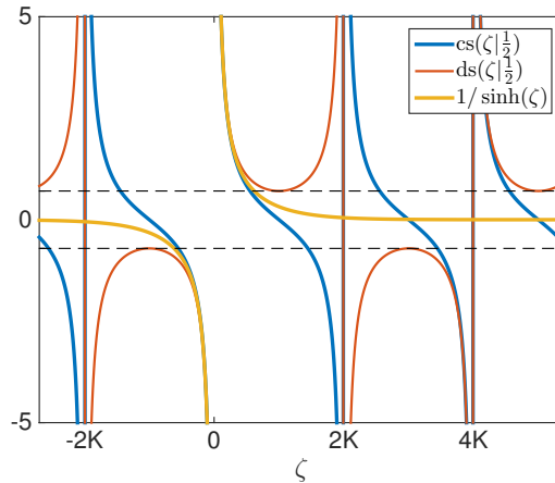
Figure 6: \operatorname{cs}(\zeta | m) , \operatorname{ds}(\zeta | m) and 1/\sinh(\zeta) for m = 1/2 . Numerically K(m) \simeq 1.85 . The horizontal dashed lines corresponds to \pm\sqrt{1-m} \simeq 0.71
