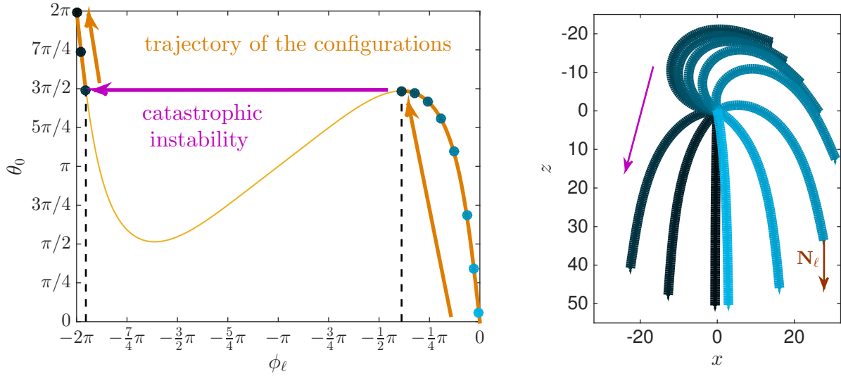
Figure 13: Left: evolution of \theta_0 according to \phi_\ell if N_\ell = 0.01 . In orange bold the history of the \phi_\ell and \theta_0 for the command \mathcal{C} . The arrows help to read the quasi static evolution and underline the gap associated to the catastrophe. Right: the successive configurations for various values of \theta_0 respecting the command \mathcal{C} . The colors of the dots in the left figure are associated to the colors of the corresponding configurations. The purple arrow highlights the brutal transition of the configurations during the catastrophe.
