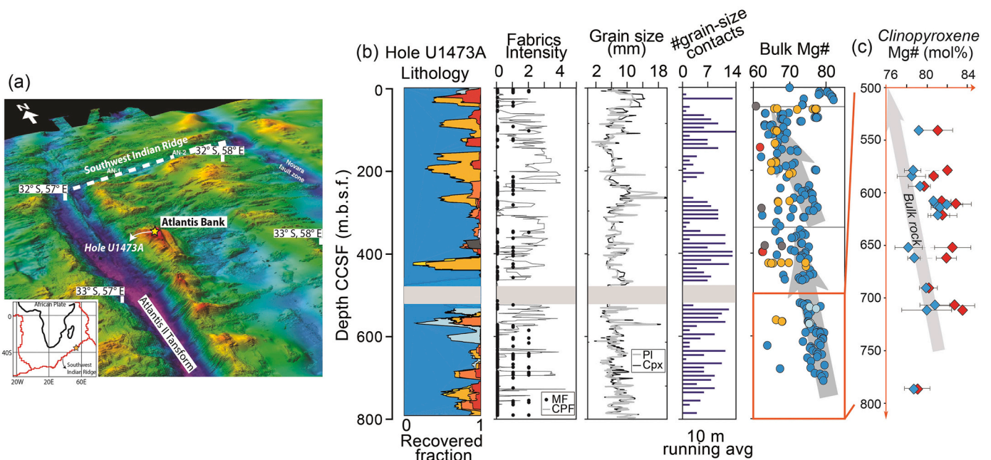
Fig. 1. (a) Location of the Atlantis Bank OCC and of IODP Hole U1473A drilled during Expedition 360 on its flat top (modified after MacLeod et al., 2017). (b) Downhole lithologies and associated textures (from left to right: magmatic (black dots) and crystal plastic fabrics (grey line, running average); Pl (light grey line) and Cpx (black line) grain sizes (mm); number of grain-size contacts, given as 10 m-running average), and downhole bulk-rock Mg# (dot colors represent the lithology as reported in the first column ‘Hole U143A Lithology’). Colors correspond to the lithology: dark blue - olivine gabbro, light blue - gabbro, yellow - disseminated oxide gabbro, orange - oxide-bearing gabbro, red - oxide gabbro, grey - diabase. The grey horizontal bar represents the drilled interval with no recovery (see MacLeod et al., 2017); (c) Composition of cores of Cpx crystals (average per sample) in the studied interval from 500 to 800 mbsf; Red diamonds represent coarse-grained Cpx, while blue diamonds display the composition of fine-grained crystals. (For interpretation of the references to colour in this figure legend, the reader is referred to the web version of this article.)
