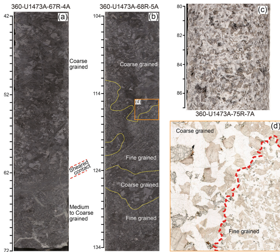
Fig. 2. Examples of grain-size variations in olivine gabbros from Hole U1473A. In (a) the contact between coarse (on top) and medium (bottom) is marked by a shear band where intense grain-size reduction is recorded; (b) Sutured and lobate, irregular grain-size contacts preserve their primary characteristics; orange box locates the thin section reported in (d); (c) Isotropic magmatic fabrics typically observed in the studied samples at the macroscopic scale; (d) Thin section showing the irregular, magmatic contact between coarse- and fine-grained olivine gabbros. Note that rock cores were cut perpendicular to the foliation plane (when visible) and possibly perpendicular to the orientation of grain-size contacts, ideally maximizing the expression of dipping structures on the cut face of the core (MacLeod et al., 2017). Therefore, the observed irregular shapes of grain-size contacts are not 2D-cutting artefacts but are rather real natural features. To observe the 3D geometry of contacts in core 360-U1473A-68R-5 see the whole round image in Supplementary Fig. S1.
