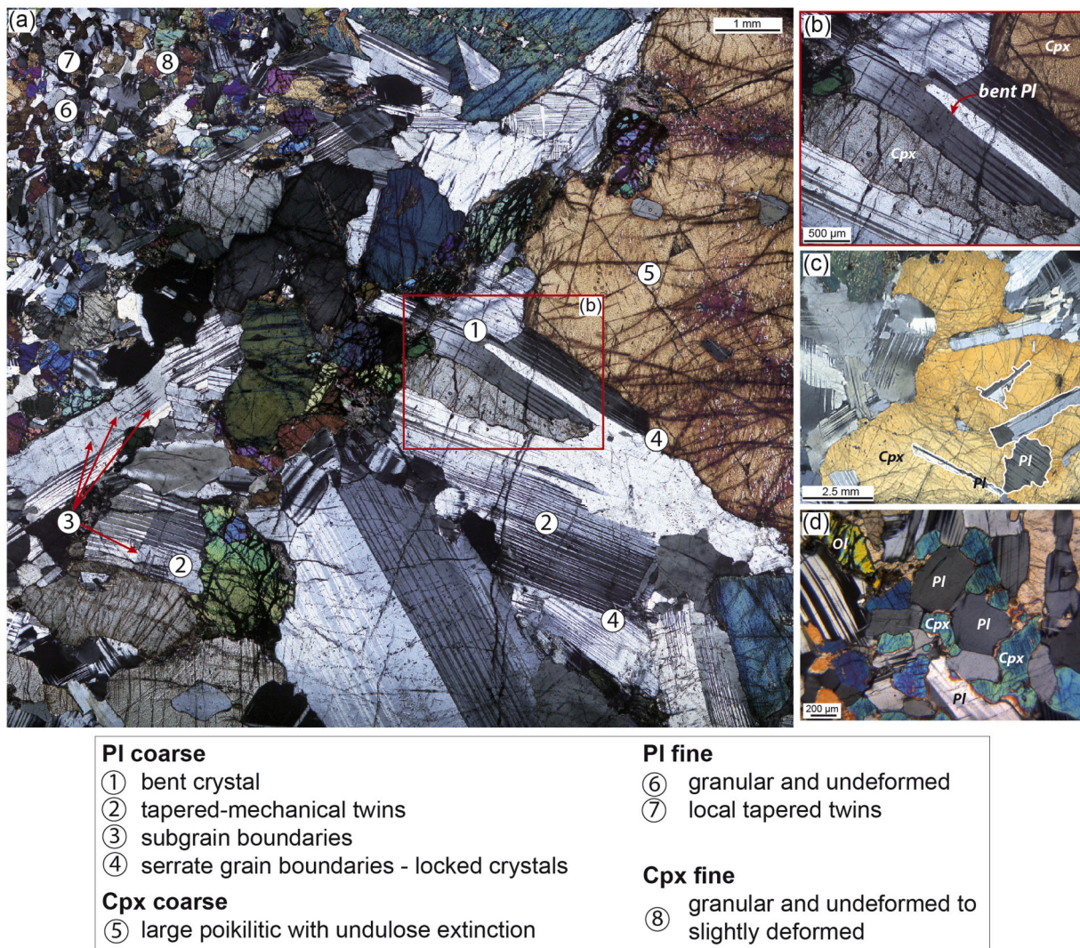
Fig. 3. Textures of coarse- and fine-grained olivine gabbros. (a) Sample 360-U1473A-66R-7 W, 12–18 cm best illustrating the characteristic textures of both coarse- and fine-grained olivine gabbros (numbers indicate the microstructures listed at the bottom of the figure); (b) Close-up showing a bent PI around Cpx; (c) Large poikilitic clinopyroxene oikocryst embaying plagioclase showing corroded grain boundaries in sample 74,360-U1473A-64R-4 W, 19–24 cm; (d) Undeformed fine-grained olivine gabbro with typical granular textures.
