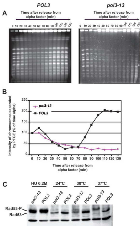
Figure 3 Evidence of persistent branched DNA structures produced during S phase that can activate DNA replication checkpoint. (A) Pulsed-field gel electrophoresis of yeast chromosomes after release from alpha factor block. POL3 and pol3-13 yeast cells were cultivated in rich medium at 24°C and arrested in G1 in presence of alpha factor. Cells were then released into YPD medium containing nocodazole to prevent next mitosis at 37°C. Time 0 corresponds to cells blocked in alpha factor just before release into fresh medium. Cells were collected every 10 minutes, and were further processed for PFGE analysis. Separated chromosomes were stained with ethidium bromide. (B) Intensity of chromosomes bands under UV light was analyzed by densitometry using ImageJ software. Densitometry value in alpha factor arrested cells was set to 100 (alpha column). Time 0 corresponds to cells blocked in alpha factor just before release into fresh medium. (C) Western blot analysis of Rad53 phosphorylation. Yeast cells were cultivated in rich medium at 24°C and arrested in G1 in the presence of alpha factor. Cells were then released into YPD medium at 24°C, 30°C, or 37°C, or at 24°C in the presence of 200 mM hydroxyurea (HU, positive control). Samples were taken at 60 minutes after release, and processed for immunoblotting to detect Rad53 with a polyclonal antibody.
