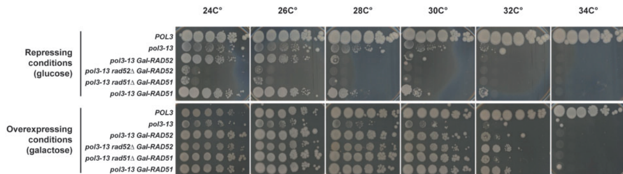
Figure 4 Increasing homologous recombination improves pol3-13 growth at nonpermissive temperature. Drop tests of serial 10-fold dilutions of yeast cell cultures on glucose-containing medium (upper row of panel, repressing conditions) and on galactose-containing medium (lower row of panel, inducing conditions). Yeast genotypes are indicated on the left. Five-microliter drops were spotted on the top of the agar plates, and cell growth was assessed after 3–4 days at indicated temperatures.
