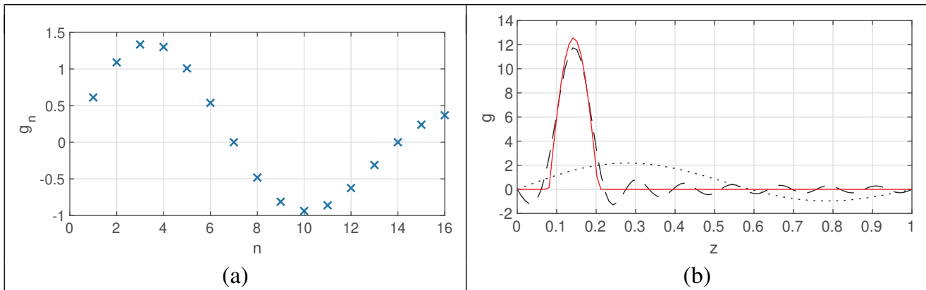
Fig. 4: Configuration 2. (a) First coefficients g_n . (b) Reference unitary spatial distribution g(z) (—) and its modal reconstructions with N = 2 modes ( \cdots ) and N = 16 modes ( --- ).
