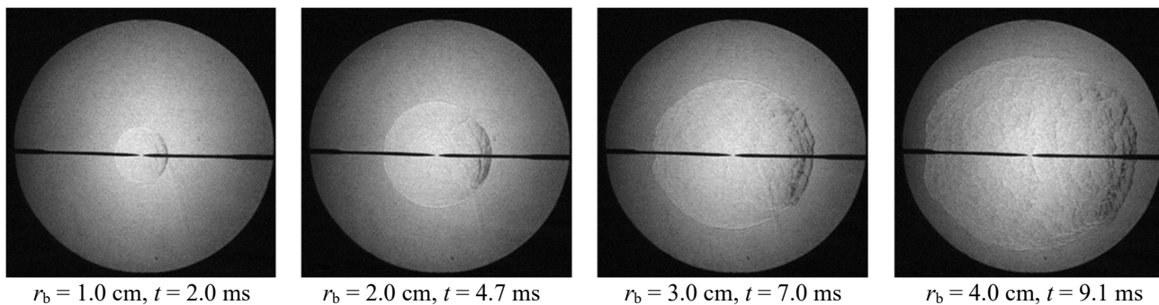
Fig. 8 Schlieren images of \text{H}_2/\text{air} flame ( \phi = 0.5 ) at ICARE
