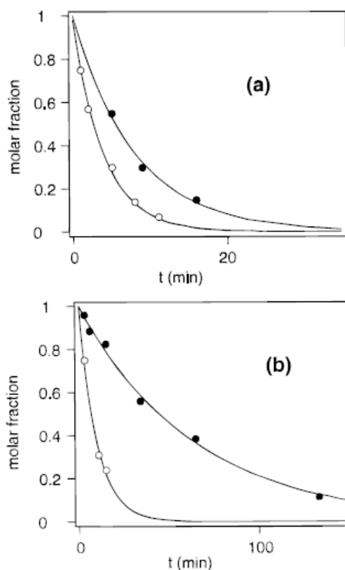
Figure 5. Decay from the EPR monitoring experiments of the relative concentration of (a) 1^+ (●) and 1^+d^3 (○) in \text{CH}_2\text{Cl}_2 at 0^\circ\text{C} and (b) 1^+ in THF at 0^\circ\text{C} (●) and 10^\circ\text{C} (○).
