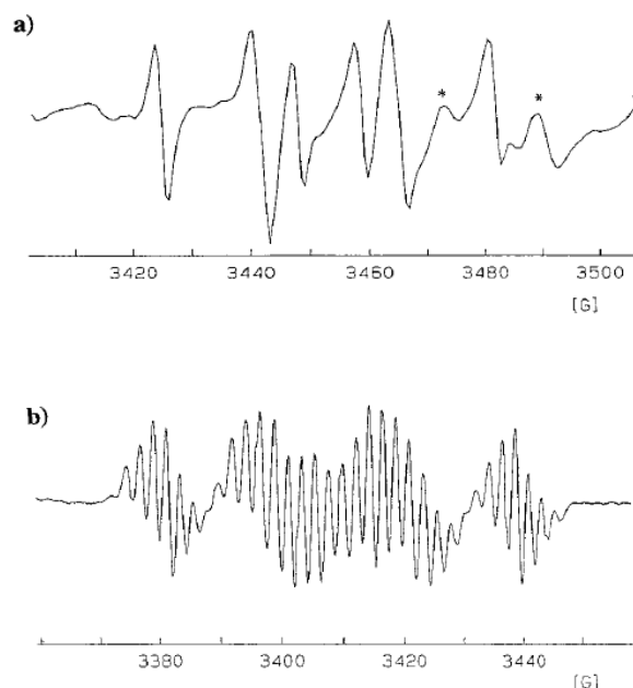
Figure 4. EPR spectrum of compound \text{Cp}^*\text{MoH}(\text{dppe})(\text{PF}_6) . Solvent = \text{CH}_2\text{Cl}_2 . (a) T = \text{room temperature} . (b) T = 0 \text{ }^\circ\text{C} . The peaks marked with an asterisk are due to an unknown impurity.
