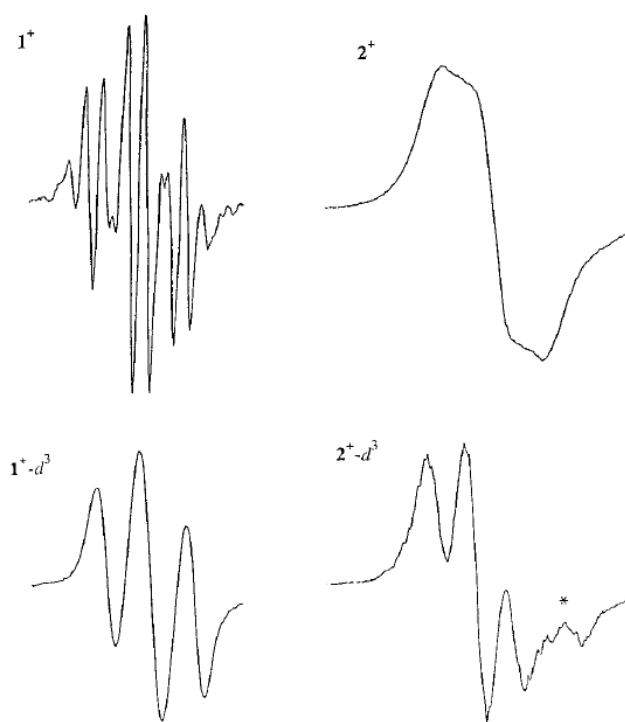
Figure 1. Room-temperature EPR spectra of compounds [Cp*MX 3 (dppe)] + (M = Mo, X = H, 1 + ; D, 1 + - d 3 . M = W, X = H, 2 + ; D, 2 + - d 3 ) in THF. The asterisk in the spectrum of 2 + - d 3 indicates an unknown impurity.
