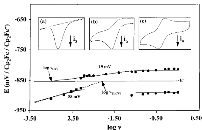
Figure 3. Peak potentials for the oxidation of 1 and reduction of 1 + in MeCN as a function of scan rate ( v in \text{V s}^{-1} ) at [\mathbf{1}] = 8.9 \times 10^{-4} M. Circles refer to CV data, and squares refer to TLCV data. The lines fitting the data are obtained from simulations as described in the text. The insets show representative thin-layer cyclic voltammograms [ v = 4 \text{ mV s}^{-1} (a)] and cyclic voltammograms [ v = 0.02 (b) and 1 (c) \text{V s}^{-1} ].
