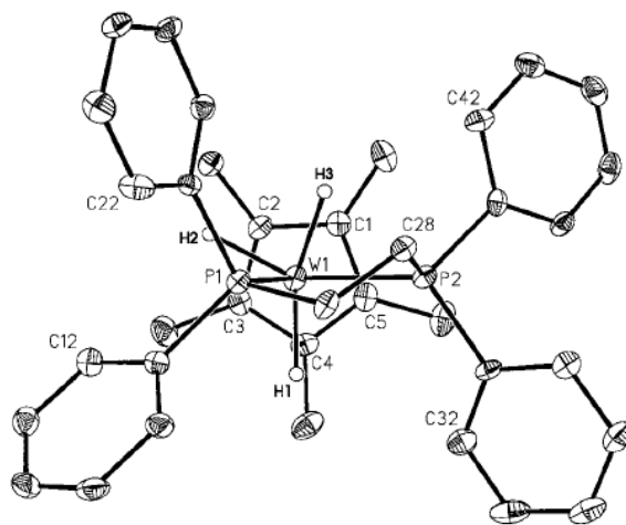
Figure 6. ORTEP view of the molecular geometry for \mathbf{2}^+ . Ellipsoids are drawn at the 30% probability level.
