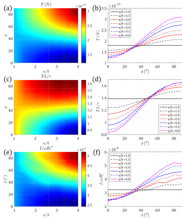
Figure 8: Influence of the cross-section at pumping. (a-b) Thrust as a function of the variable space \{\frac{a}{b}, \phi\} . (c-d) Normalized thrust per torque ( \frac{TL}{\tau} ). (e-f) Normalized flux ( \frac{I}{\omega R_c^3} ).
