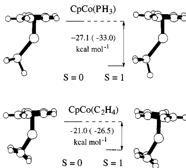
Figure 1. Relative energies of singlet and triplet [CpCo(PH 3 )] and [CpCo(C 2 H 4 )]; \Delta E_{S-T} calculated at the B3LYP/6-3111G(2d,2p) level of theory, with B3LYP/LanL2DZ values indicated in parentheses.
