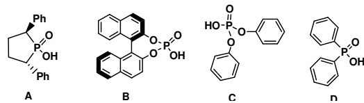
Figure 2. Catalysts structures
