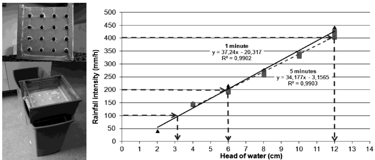
Figure 3. (Left) Pictures of the Portable Laboratory Rainmaker (PLR) and (right) its calibration line.
