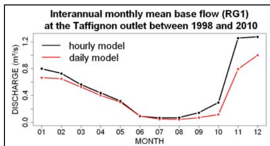
Figure 9 : Comparison of interannual monthly mean hourly and daily base flow.
