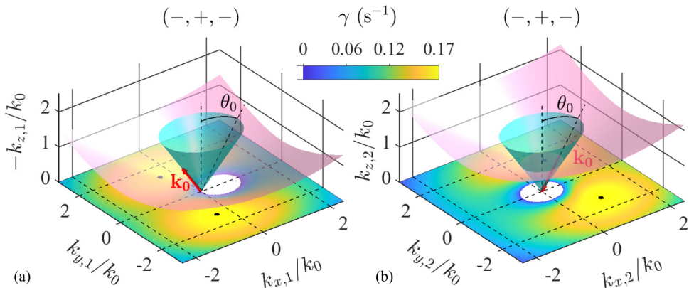
FIG. 2. Resonance surfaces of (a) \mathbf{k}_1 and (b) \mathbf{k}_2 for the combination of wave polarities (-, +, -) and a primary wave defined by k_0 = 0.83 \text{ rad cm}^{-1} , s_0 = -1 , \sigma_0^* = 0.84 , and b_0 = 0.39 \text{ cm s}^{-1} . In (a) the vertical axis shows -k_{z,1} for the sake of clarity. The two 3D plots also show the cone of apex at \mathbf{k}_i = \mathbf{0} and of semiangle \theta_0 = \cos^{-1}(\sigma_0^*) . This cone represents the waves at the forcing frequency according to the dispersion relation. Below each resonance surface, we also report the map of the growth rate \gamma of the instability in the plane (k_{x,i}, k_{y,i}) in which the locations of the maximum growth rate are shown by black dots. The value \nu = 1.20 \times 10^{-6} \text{ m}^2 \text{ s}^{-1} is used for the kinematic viscosity in order to match the experimental value in the next section.
