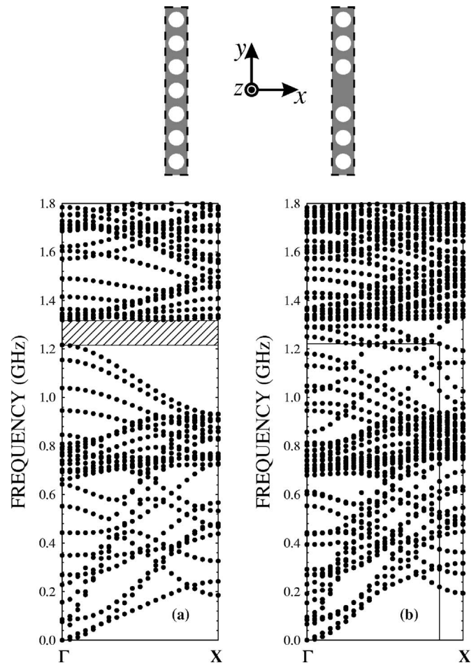
FIG. 3. Band structure along the \Gamma X direction calculated with a supercell containing 1 \times 7 unit cell, for (a) the perfect phonic crystal plate and (b) the phonic crystal plate containing a waveguide formed by filling the hole in the fourth unit cell. The inset depicts the 1 \times 7 supercell considered in each case. The two straight lines indicate the location of the guided mode analyzed in Fig. 4.
