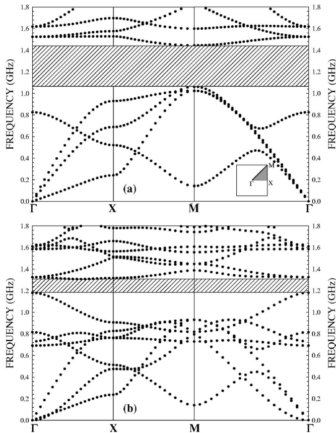
FIG. 2. Elastic band structures calculated with the finite element method for (a) the bulk 2D phonic crystal (structure of infinite extent along the three spatial directions) and (b) the freestanding phonic crystal plate of thickness h=a=0.77 \mu\text{m} made of a square array of holes drilled in a PZT 5A piezoelectric matrix with \beta=0.7 . The inset represents the first Brillouin zone ( \Gamma XM ) of the square array. The components of the wave vector at the \Gamma , M , and M points are (0,0) , (\pi/a,0) , and (\pi/a,\pi/a) , respectively, with \pi/a=4.08 \mu\text{m}^{-1} .
