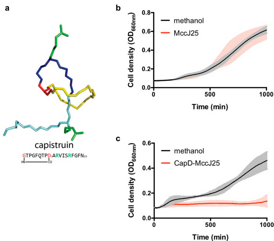
Figure 5. Functional characterization of CapD in the presence of MccJ25. (a) Structure of capistrain. Capistrain belongs to the class II lasso peptide RiPPs. Coloring as in Figure 1a. (b) Growth of drug-hypersensitive E. coli \Delta acrAB expressing MccJ25 and (c) CapD in the presence (red) or in the absence (black) of MccJ25 (10 \mu M). In the presence of MccJ25, the cells grow to high density, whereas cells expressing CapD cannot confer self-immunity to MccJ25 that prevents cell growth due to the inhibition of the RNA polymerase.
