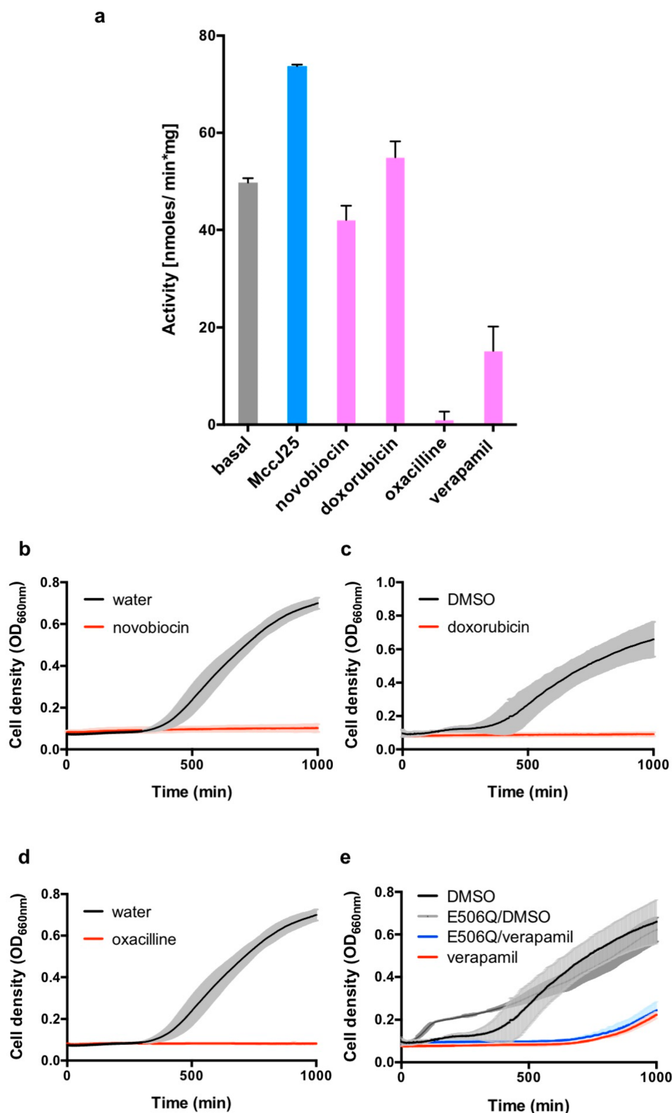
Figure 4. Functional characterization of McdJ in the presence of different drugs. (a) The basal ATPase activity of McdJ is induced by MccJ25 (same data used as in Figure 3b for clarity) but not by other drugs. Error bars are shown for all measurements (mean \pm SEM; n = 3 ). (b) Growth of drug hypersensitive E. coli \Delta acrAB expressing McdJ with (red) or without (black) novobiocin ( 5 \mu\text{g mL}^{-1} ), (c) doxorubicin ( 5 \mu\text{g mL}^{-1} ), (d) oxacillin ( 5 \mu\text{g mL}^{-1} ), and (e) verapamil ( 450 \mu\text{g mL}^{-1} ). The E506Q mutant was used to assess if the delayed cell growth in the presence of verapamil was due to McdJ active transport; the E506Q growth curves are blue with and black without verapamil. All cytotoxicity assays were performed in triplicate from three different colonies. The curves represent the mean of three independent experiments.
