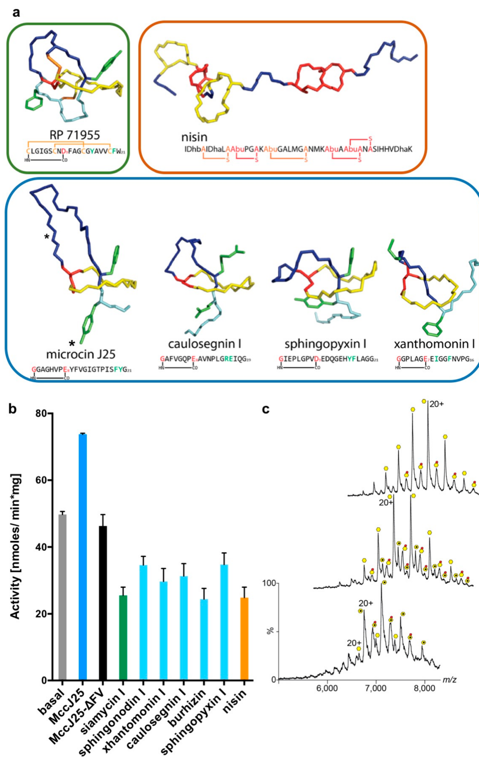
Figure 3. Functional characterization of MccJ25 in the presence of different RiPPs. (a) Overview of all available 3D structures of peptides used in this study. The lasso peptides (MccJ25 (PDB code 1Q71), RP 71955 (PDB code 1RPB), caulosegnin I (PDB code 2LX6), sphingopyxin I (PDB code 5JQF), xanthomonin I (PDB code 4NAG)) are color coded as in Figure 1. Disulfide bonds are in orange. The lantipeptide nisin (PDB code 1WCO) is color coded by residues outside of the (methyl)lanthionone rings (blue) and the rings itself (alternating yellow and red); Dha = dehydroalanine, Dhb = dehydrobutyrine, Abu = aminobutyryne. RP 71955 was used to represent the closely related siamycin I structure (the only differences in primary structures are found at position 4 (Val for siamycin I, Ile for RP71955) and position 17 (Ile for siamycin I, Val for RP71955)). Each RiPP structure is boxed in different color; green for class I, blue for class II, and orange for the lantipeptide. (b) The basal ATPase activity of MccJ25 is induced by MccJ25 but not by other RiPPs. The bars are color coded to distinguish between the different RiPPs classes as in panel (a). Error bars are shown for all measurements (mean \pm SEM; n = 3 ). (c) Mass spectrum of MccJ25 reveals two series of charge state peaks consistent with apo MccJ25 and LPS bound adduct with 20+ main charge state (top panel). Addition of MccJ25- \Delta FV (middle panel) and MccJ25 (bottom panel) at a final concentration of 8 \mu M to MccJ25 leads to the formation of a complex with protein and LPS bound peaks. A much higher degree of complex formation is observed for MccJ25 than MccJ25- \Delta FV. Deconvoluted masses of apo, LPS, and peptide bound peaks are in agreement with theoretical masses. Apo MccJ25, LPS bound MccJ25, and
