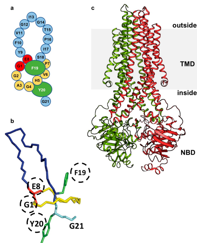
Figure 1. Structures of MccJ25 and McjD. (a) Schematic of the lasso topology of MccJ25. Its amino acid sequence is shown in a ball model. (b) Three-dimensional NMR structure of MccJ25 (PDB 1Q71). 7 The macrolactam ring, the isopeptide bond between the G1 amino group and the E8 side chain carboxylate, the Y9–S18 loop region, and the two bulky aromatic residues F19 and Y20 serving as a lock for maintaining the lasso topology are in yellow, red, blue, and green, respectively (as in panel a). (c) Crystal structure of apo-McjD (PDB 5OFP). 15 The two monomers are shown as green and red cartoons, and the membrane is depicted as a gray box.
