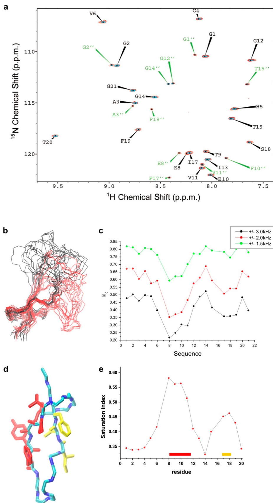
Figure 2. NMR analysis of the MccJ25–McJd interaction. (a) CEST ^1\text{H} – ^{15}\text{N} HSQC experiments of MccJ25 in phosphate buffer measured at 310 K using an 800 MHz instrument with a cryoprobe TCI. Cyan and red spectra report the CEST measured with an offset of 1.5 kHz and 100 kHz, respectively. Individual CEST profiles are shown in Supporting Information Figure 3 and control experiments with MccJ25 and bicelles are shown in Supporting Information Figure 6. (b) Chemical-shift refined structures of MccJ25 in its main primary (black) and secondary (red) conformations
