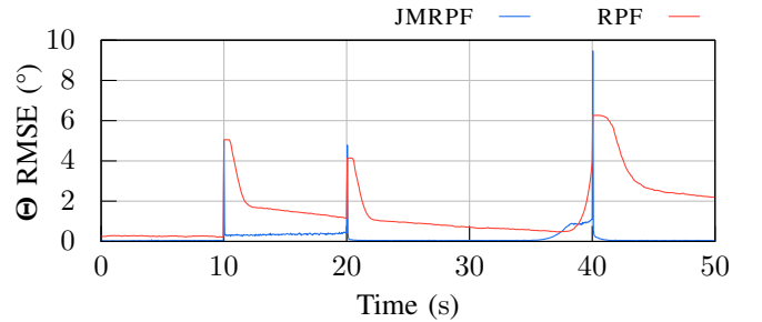
Fig. 5. RMSE of the pitch sensor fault
