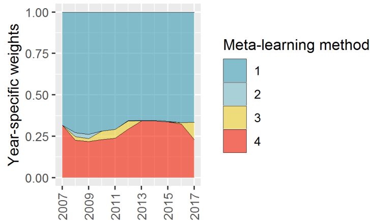
Figure 2: Evolution (from 2007 onward) of the weights attributed by the overarching Super Learner to 4 of its base algorithms, each one a Super Learner itself using its own meta-learning method. The other base algorithms get no weight at all (on this time window).
