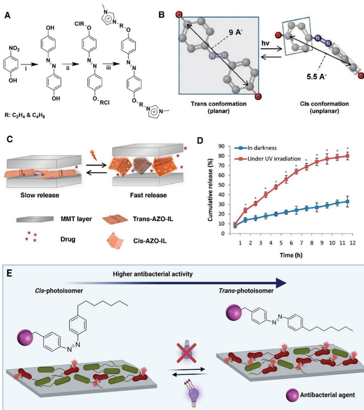
Figure 15. Light-responsive drug delivery nanoplatfrom containing azobenzene imidazolium ionic liquid acting as molecular jacks. A) Synthesis of 4,4'-bis(2-ethoxymethylimidazolium)azobenzene ionic liquid (Azo-ILs). B) Switching the molecular jacks from the cis-state to the trans-state alters the basal distance between exfoliated montmorillonite (MMT) clay layers and creates room for drug-loaded (release triggered by ultraviolet light radiation). C) Schematic of the intercalation between Azo-ILs and MMT layers D) In vitro release profiles of para -aminobenzoic acid in the dark (blue) and upon ultraviolet light radiation (red). Reproduced with permission. [137] Copyright 2018, American Chemical Society. E) Schematic illustration on antibacterial activity of cis - and trans -states of azo molecule. In most cases trans -state of azobenzene derivatives containing antibacterial agents perform better than their cis -states. However, in this case, it is predicted that the cis -state of azobenzene imidazolium ionic liquid acts more efficient than trans -state due to the availability of imidazolium cations in the increased basal distance of MMT nanolayers.
